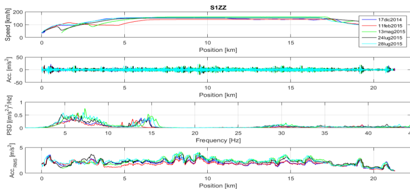
Figure 5: Monitoring of track state for the Torino – Genova line from December 2014 to July 2015
