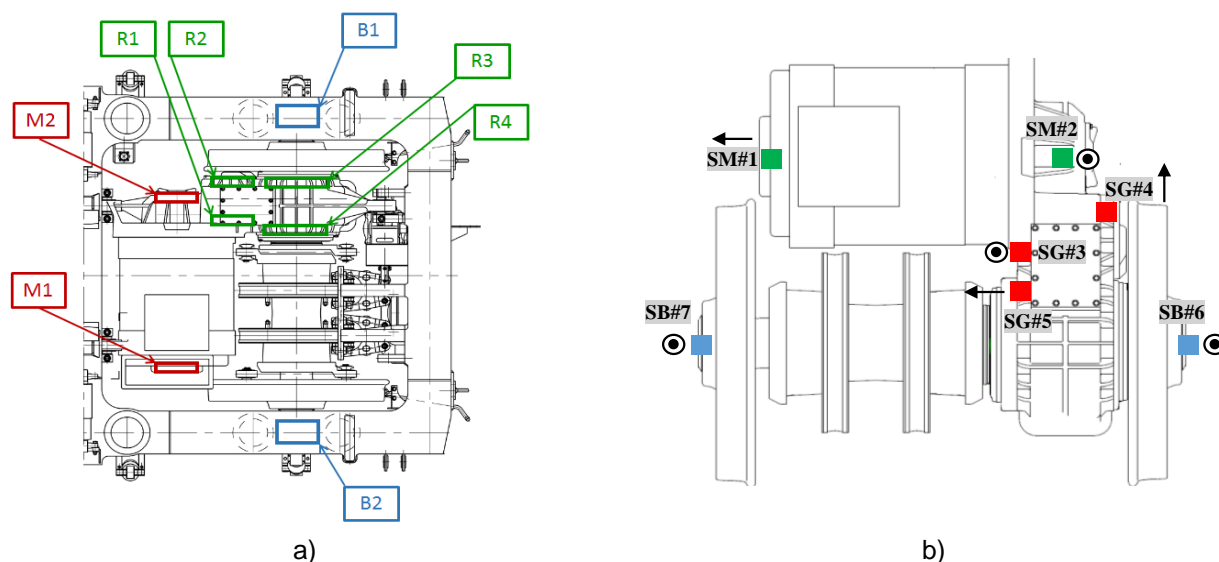
Figure 1. a) bearings of the traction monitoring unit. b) position of the sensors
