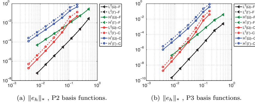
FIGURE 5.5. Error norms vs the mesh step computed for the 2D test cases with the Isogeometric Analysis discretization. The notations -F and -C stand for Flat and Curved \Gamma_1 , respectively.
