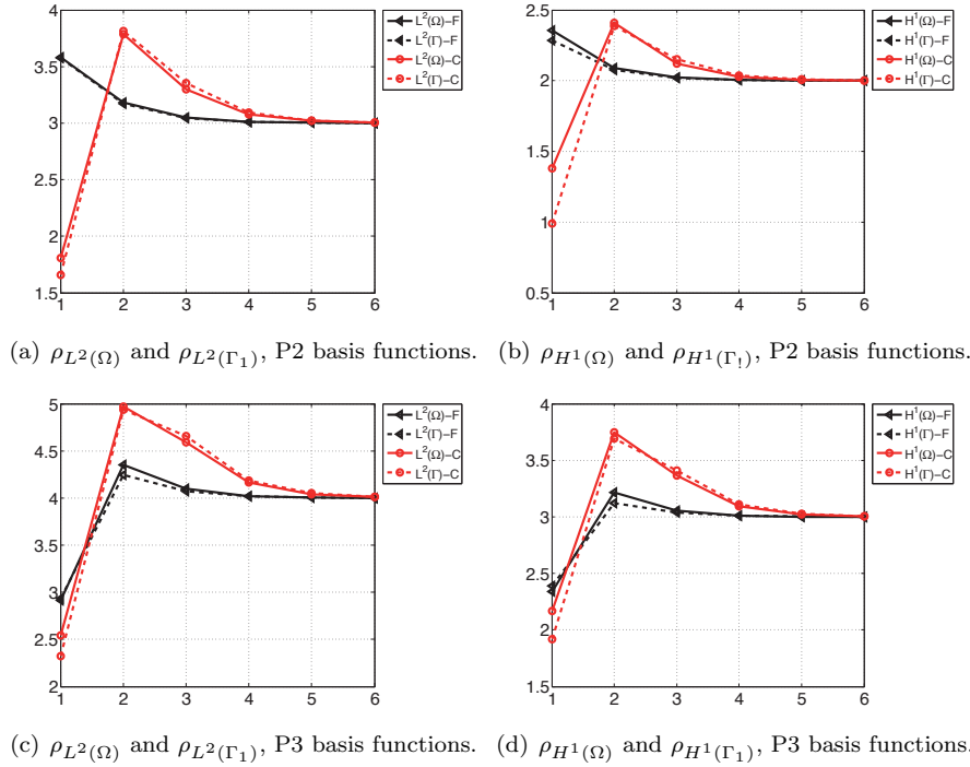
FIGURE 5.6. Rate of convergence on the refinement step computed for the 2D test cases with the Isogeometric Analysis discretization. The notations -F and -C stand for Flat and Curved surface \Gamma_1 , respectively.
