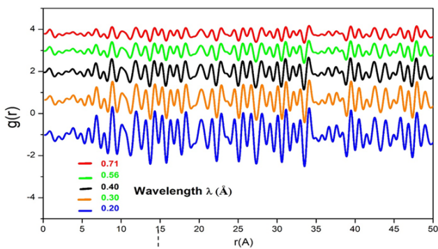
Fig.1: Effect of wavelength on XRD patterns.
