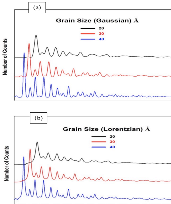
Fig.10: Effect of crystallite size on XRD diffractograms for: (a) Gaussian distribution and (b) Lorentzian distribution.
