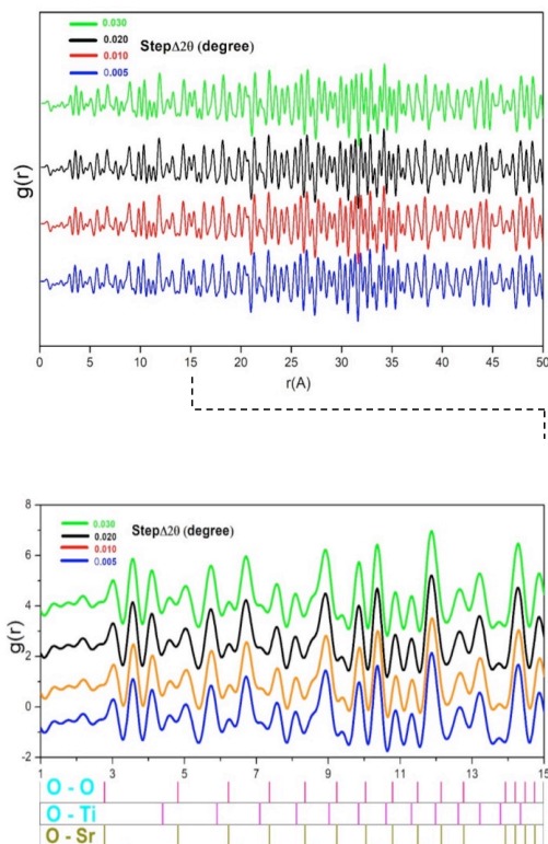
Fig.7: Effect step size on PDF plots.
