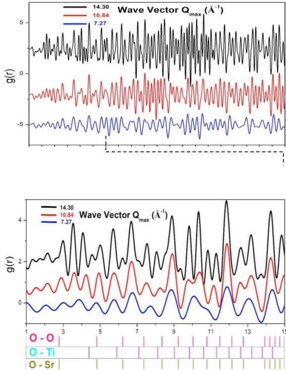
Fig.4: Effect of wave vector on PDF plots considering conventional source.
