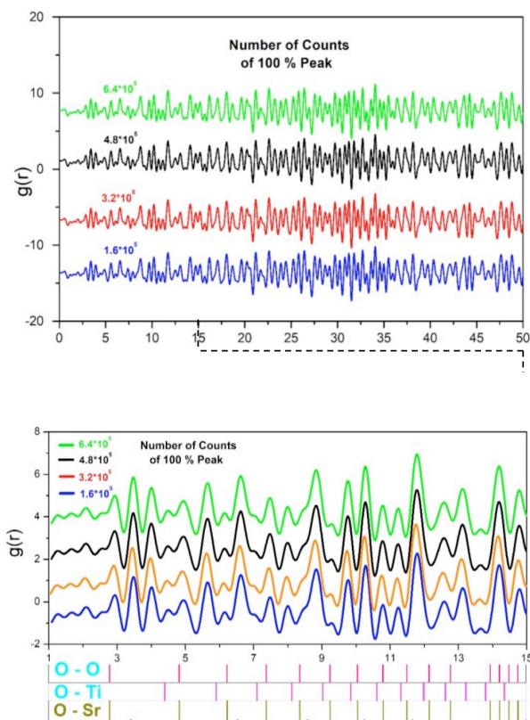
Fig.17: Effect of number of counts on PDF plots.
