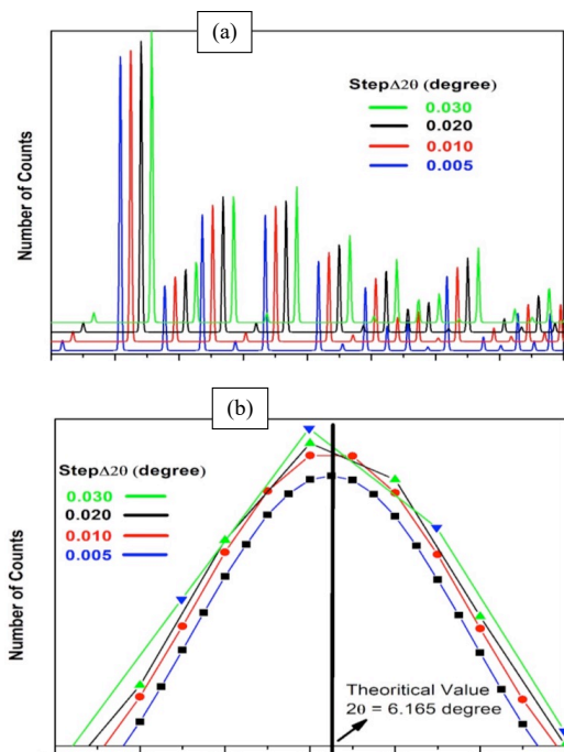
Fig.6: Effect of step size at constant wavelength and Qmax on: (a) Diffraction pattern and (b) 100% peak position.
