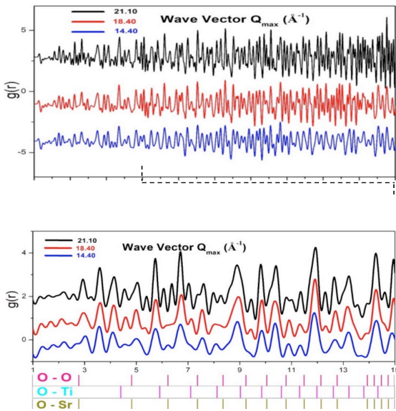
Fig.5: Effect of wave vector on PDF plots considering conventional source.
