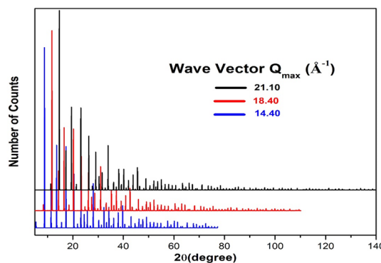
Fig.3: Effect of Q_{max} on XRD patterns considering:
