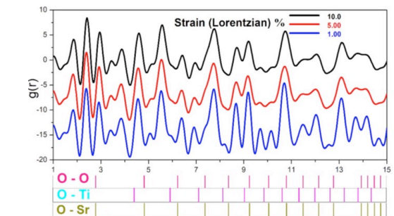
Fig.15: Effect of residual strain for Lorentzian distribution on PDF plots.
