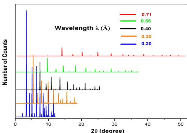
Fig.1: Effect of wavelength on XRD patterns.
