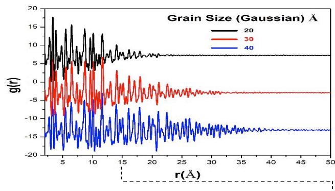
Fig.11: Effect of crystallite size for Gaussian distribution on PDF plots.
