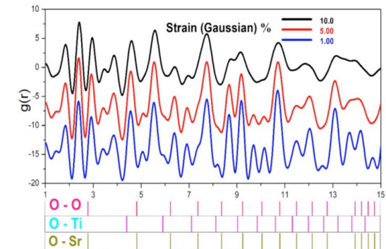
Fig.14: Effect of residual strain for Gaussian distribution on PDF plots.
