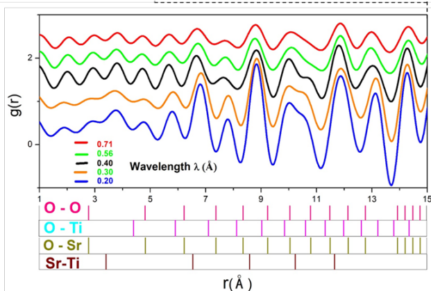
Fig.2: Effect of wavelength on: PDF plots.
