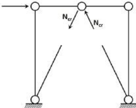
Figure B.7 - Static scheme for the standard interpretation of V-bracing system
