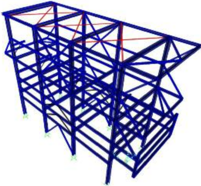
Figure B.2 - Modified layout, with horizontal cross-bracing on the top level.
