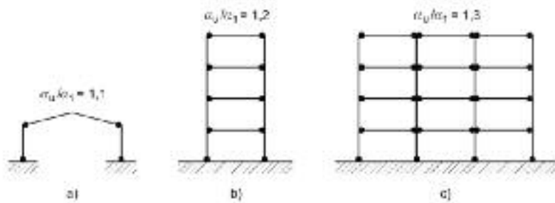
Figure B.5 - Moment resisting frames (dissipative zone in beam and at bottom of column). Default value for \alpha_{u1}/\alpha_1 (see 6.3.2(3) and Table 6.2)
