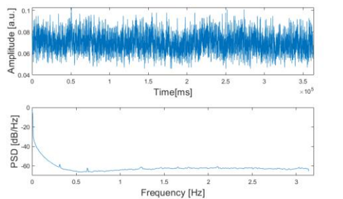
Fig. 7. Periodogram of changes in flame luminosity for stable flame in area E
