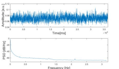
Fig. 6. Periodogram of changes in flame luminosity for stable flame in area D
