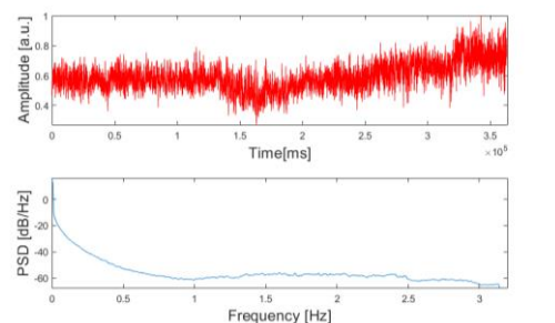
Fig. 9. Power spectral density for measured data from variant II in area B
