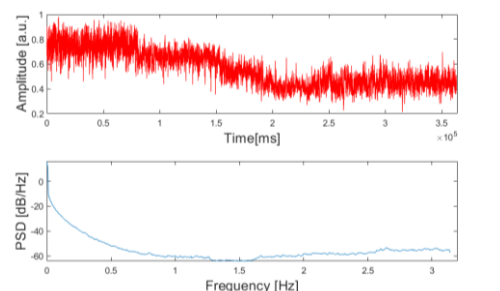
Fig. 10. Power spectral density for measured data from variant II in area C
