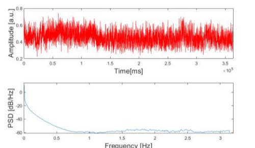
Fig. 11. Power spectral density for measured data from variant II in area D
