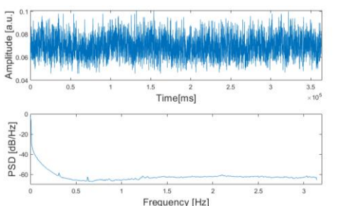
Fig. 5. Periodogram of changes in flame luminosity for stable flame in area C
