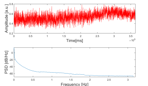
Fig. 8. Power spectral density for measured data from variant II in area A
