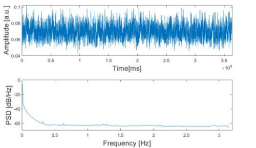
Fig. 3. Periodogram of changes in flame luminosity for stable flame in area A
