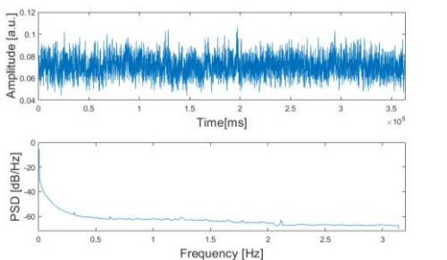
Fig. 4. Periodogram of changes in flame luminosity for stable flame in area B
