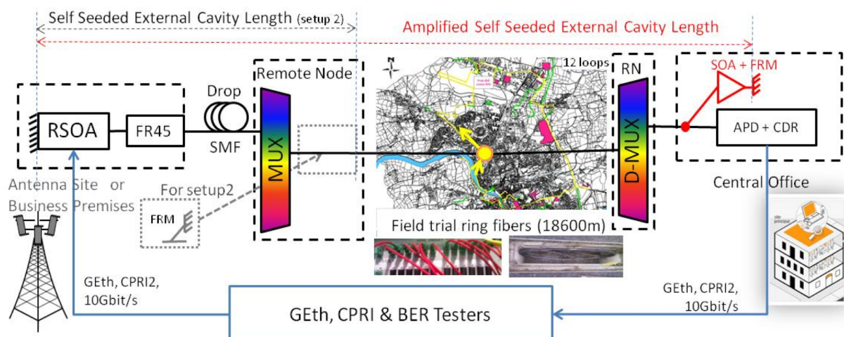
Fig. 1: Experimental setup: amplified self-seeded field trial setup and self-seeded setup using a partial mirror at RN (setup 2)
