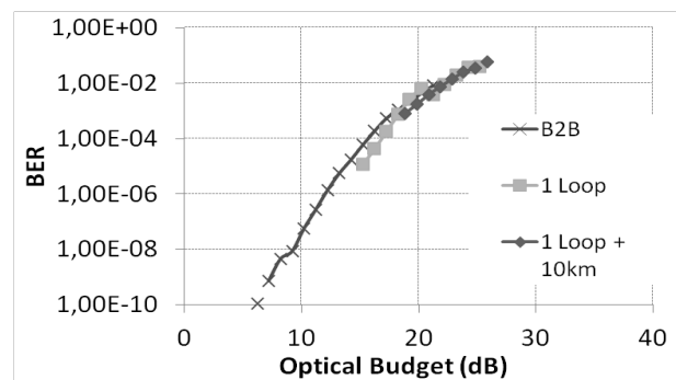
Fig.7: 10-Gbit/s BER results according to the transmission fiber length for a 10-m cavity length ( 2^7-1 PRBS) vs OB.
