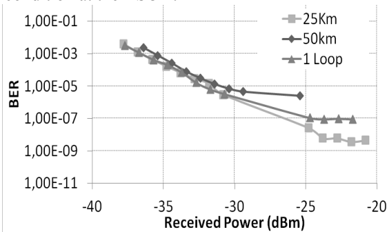
Fig. 4: 2.5 Gb/s BER results vs received power with 25 km (gray squares), 50 km (black diamonds) SSMF and 1 field trial loop (18600m, gray triangles) for a 2^{31}-1 PRBS
