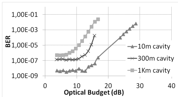
Fig. 5: BER results according to cavity length at 2.5Gbit/s ( 2^{31}-1 PRBS) for back-to-back transmission.
