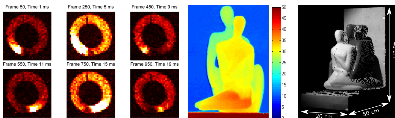
Fig. 1. Left: Acquisition of a gas discharge inside a fluorescent lamp at 50,000 fps in photon counting mode. Center: 3D scanned scene acquired in photon timing mode, where distance is expressed in centimeters. Right: The SPAD camera allows a simple 2D+3D merge and scanning, as shown with this small statue with 51 kpixel lateral resolution and 5 mm depth resolution, acquired at 8 m distance.
