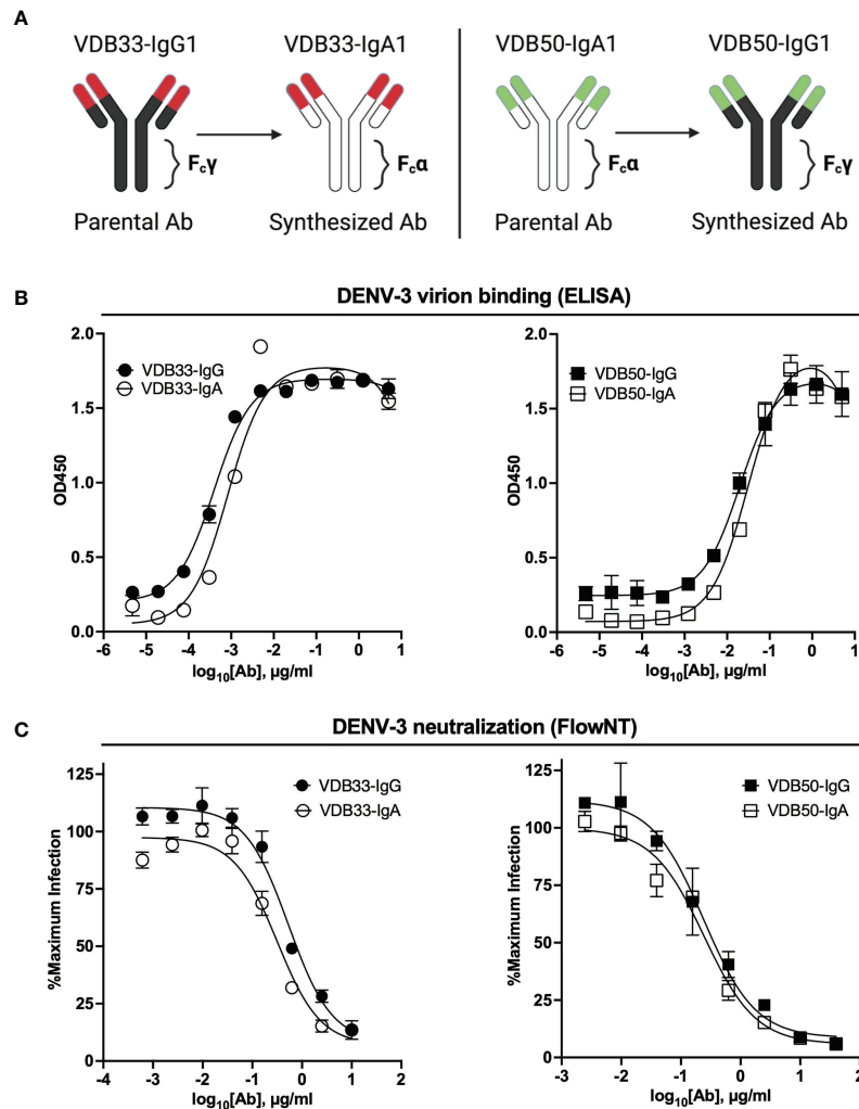
FIGURE 1 | Isotype conversion scheme, DENV binding, and DENV neutralization capacity of VDB33 and VDB50 mAbs. (A) Schematic of isotype conversion of VDB33 and VDB50 from respective parental isotypes, indicating conservation of antigen-binding domains and alteration of Fc domains. (B) DENV-3 binding capability of VDB33-IgG, VDB33-IgA, VDB50-IgG, and VDB50-IgA measured by DENV virus-capture ELISA. (C) DENV-3 neutralization capability of VDB33-IgG, VDB33-IgA, VDB50-IgG, and VDB50-IgA as assessed by FlowNT. Neutralization data are presented as a percent of the positive (no neutralizing mAb) control for each replicate. Error bars \pm SEM. Data are representative of at least 4 independent experiments.
