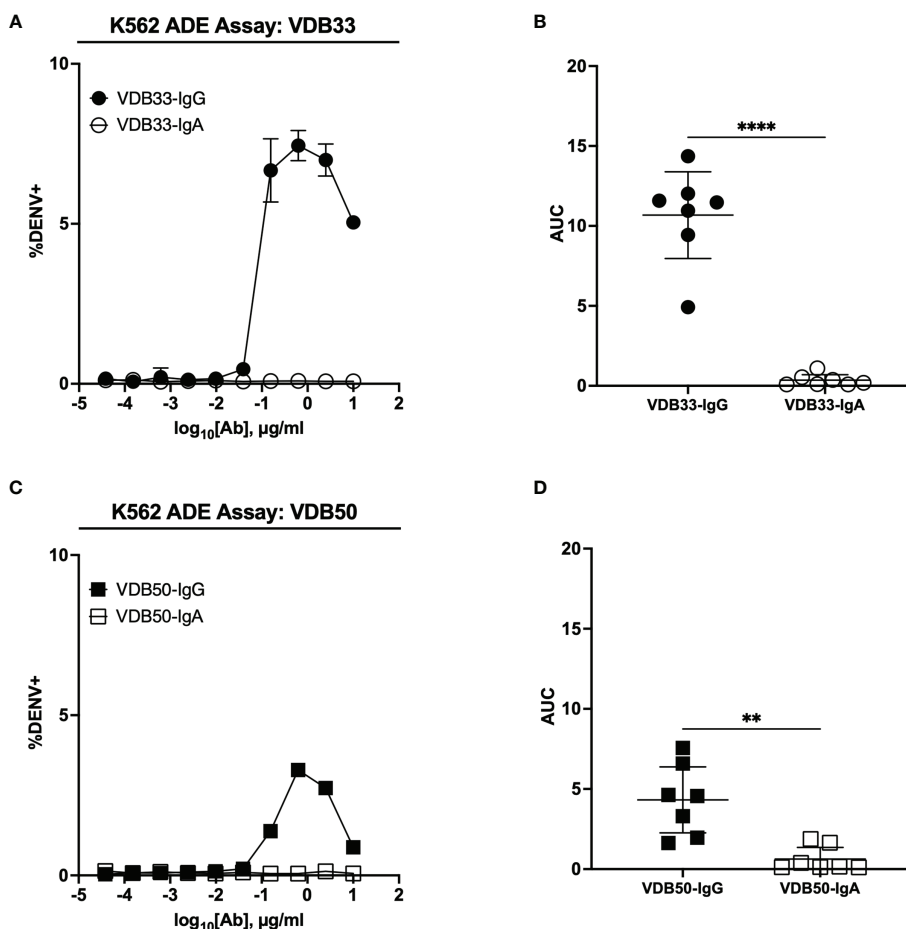
FIGURE 2 | ADE activity of DENV-reactive IgG and IgA isotype antibodies. (A) ADE activity of VDB33-IgG and VDB33-IgA against DENV-3 in K562 cells. (B) AUC values of 7 independent experimental replicates of DENV-3 ADE assay with VDB33-IgG and VDB33-IgA (C) ADE activity of VDB50-IgG and VDB50-IgA against DENV-3 in K562 cells. (D) AUC values of 7 independent replicates of DENV-3 ADE assay with VDB50-IgG and VDB50-IgA. Error bars +/- SEM. ** p < 0.01 , **** p < 0.0001 , unpaired t test. Data are representative of at least 7 independent experiments.
