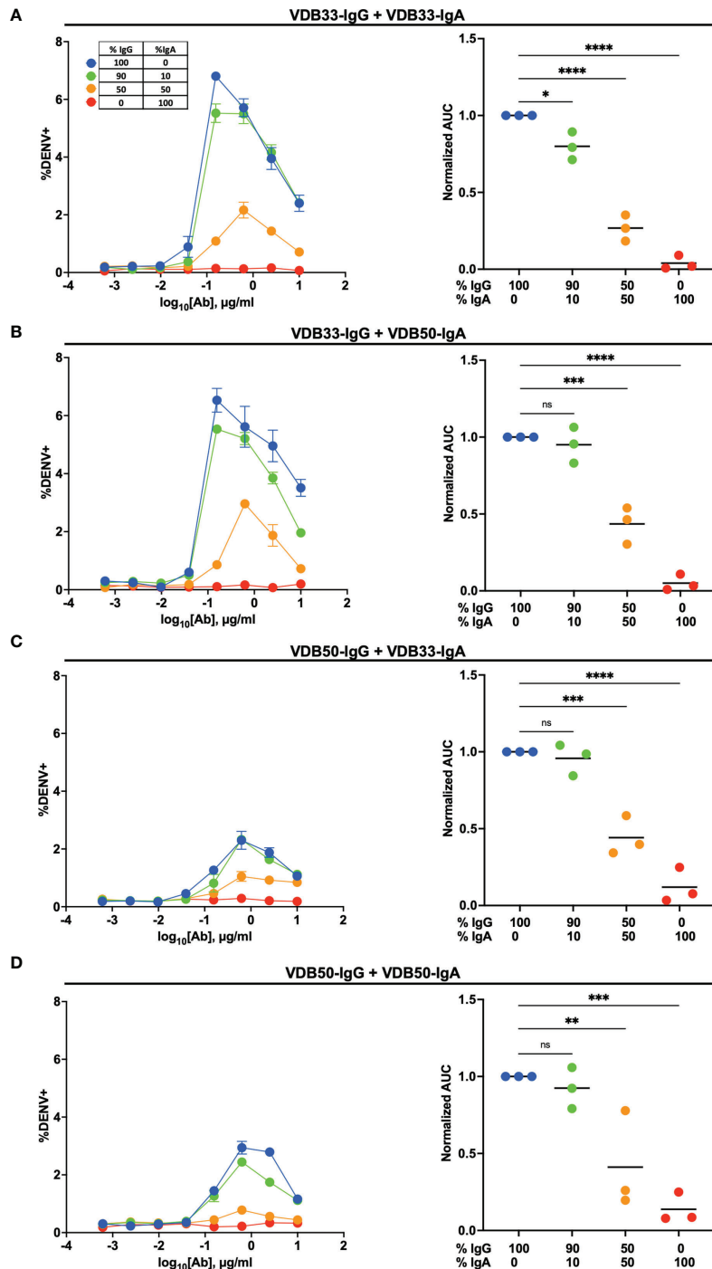
FIGURE 3 | Homotypic and heterotypic monoconal IgA antagonizes IgG-mediated antibody-dependent enhancement. (A) DENV-3 ADE activity of VDB33-IgG when antagonized with VDB33-IgA. Total antibody concentration for each dilution point was held constant, with varying ratios of VDB33-IgG and VDB33-IgA as indicated. AUC of each ADE titration was calculated and normalized to that of the 100% IgG condition. (B) DENV-3 ADE activity of VDB33-IgG when antagonized with VDB50-IgA. The AUC of each ADE titration was calculated and normalized to that of the 100% VDB33-IgG condition. (C) DENV-3 ADE activity of VDB50-IgG when antagonized with VDB33-IgA. AUC of each ADE titration was calculated and normalized to that of the 100% VDB50-IgG condition. (D) DENV-3 ADE activity of VDB50-IgG when antagonized with VDB50-IgA. AUC of each ADE titration was calculated and normalized to that of the 100% VDB33-IgG condition. Blue = 100% IgG/0% IgA. Green = 90% IgG/10% IgA. Orange = 50% IgG/50% IgA. Red = 0% IgG/100% IgA. "ns" denotes "non-significant" ( p > 0.05 ). * p < 0.05 , ** p < 0.01 , *** p < 0.001 , **** p < 0.0001 1-way ANOVA with Dunnett correction for multiple comparisons. Data are representative of at least 4 independent experiments.
