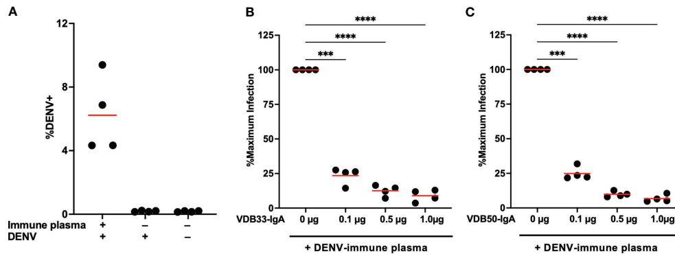
FIGURE 4 | Monoclonal IgA antagonizes ADE mediated by polyclonal DENV-immune plasma. (A) DENV immune plasma enhances DENV-3 infection of K562 cells. Each datapoint represents a unique plasma donor ( n = 4 ). (B) VDB33-IgA antagonizes in vitro enhancement of DENV-3 infection mediated by polyclonal DENV-immune serum. Serum used at a 1:50 dilution for ADE assay, n = 4 unique plasma donors. The percentage of DENV-positive cells was normalized to that observed in the plasma-only condition. (C) VDB50-IgA antagonizes in vitro enhancement of DENV-3 infection mediated by polyclonal DENV-immune serum. Serum used at a 1:50 dilution for ADE assay, n = 4 unique plasma donors. The percentage of DENV-positive cells was normalized to that observed in the plasma-only condition. *** p < 0.001 , **** p < 0.0001 1-way ANOVA with Dunnett correction for multiple comparisons. Data are representative of at least 4 independent experiments.
