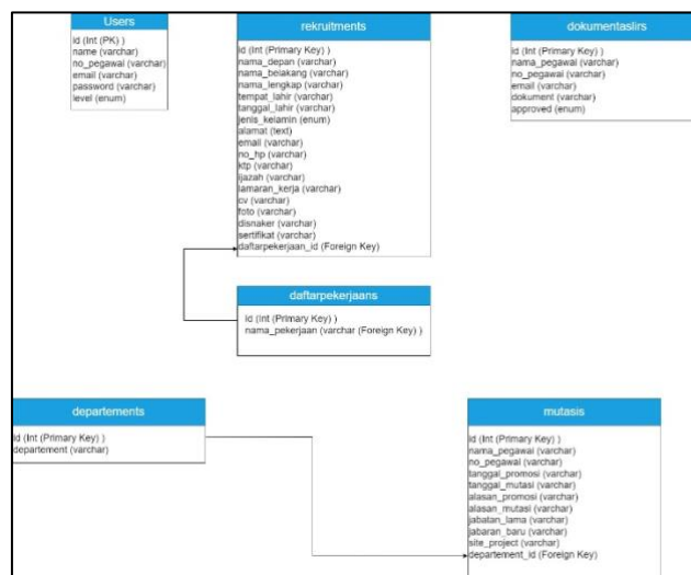
Gambar 11. Class Diagram
