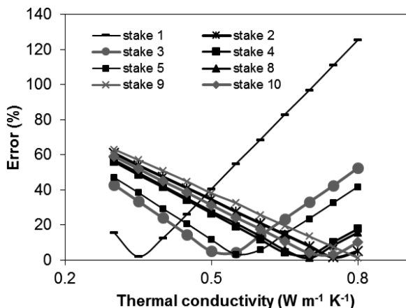
FIG. 9 - Error (%), difference between calculated and measured total ablation by varying the thermal conductivity values.
