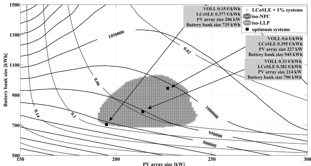
Fig. 6. Area comprising the systems with LCoSLE at the most 1% bigger than optimum LCoSLE for VOLL 0.33 €/kWh, and optimum systems for VOLL 0.15 and 0.6 €/kWh.
