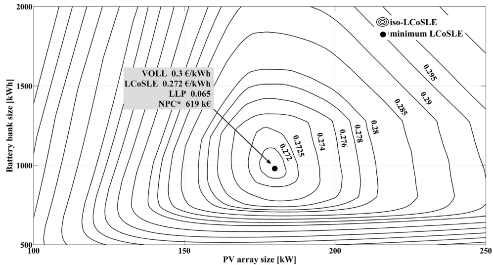
Fig. 1. LCoSLE function trend and minimum.
