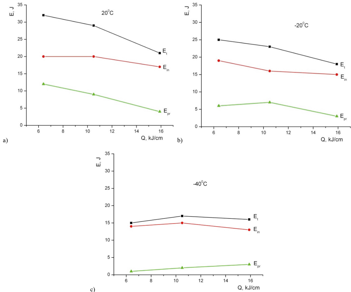
Fig. 1. Dependence total impact energy, crack initiation energy and crack propagation energy vs. heat input at: a) 20^\circ\text{C} ; b) -20^\circ\text{C} ; c) -40^\circ\text{C}
