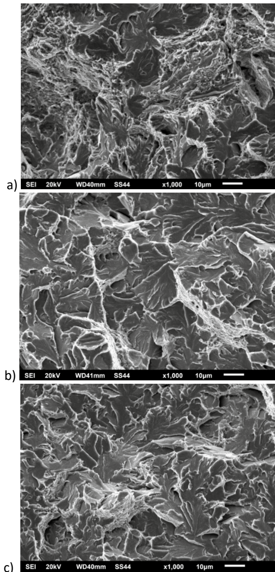
Fig.2. Fractography of Charpy specimens from the central zone of fracture at room temperature: a) sample 1 (6.4 kJ/cm); b) sample 2 (10.5 kJ/cm); c) sample 3 (15.9 kJ/cm)
