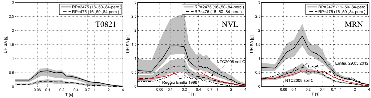
Figure 5 – Percentile Uniform Hazard Spectra calculated for the study sites with Logic Tree of Figure 4. Low UHS at T0821 depend on corresponding low \delta S2S values (see Figure 3). Dash-dot curves for MRN and NVL are spectra from actual records (1996 and 2012), while red curves are Italian code spectra (NTC2008) for Eurocode 8 class C subsoil, 475 years return period.
