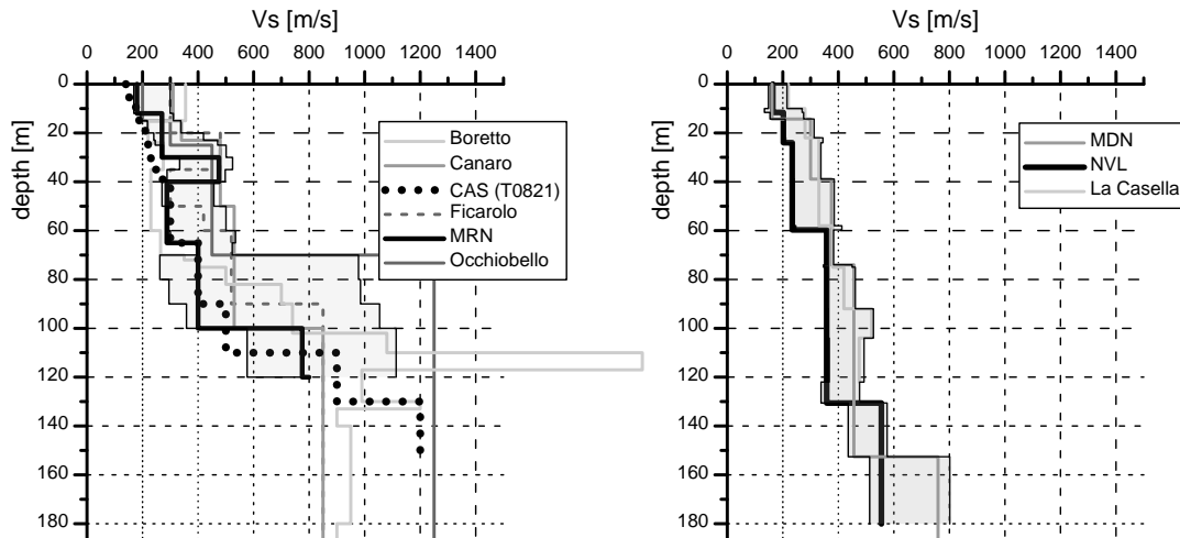
Figure 2 – Representative types of V_s profiles in Po Plain: ( left ) with strong impedance contrast at 80-to-120 m depth, ( right ) without strong contrast in the upper 200 m. (Faccioli et al. 2015).
