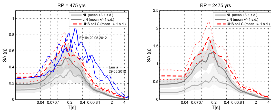
Figure 6 – Response spectra from linear (dark grey, shaded) and fully non-linear (light grey, shaded) analyses and UHS for class C soil (red lines) yielded by the one-step fully probabilistic approach (see Figure 5). Stdrd. dev. values of NL and LIN curves are the \sigma_{TOT} of Table 1.
