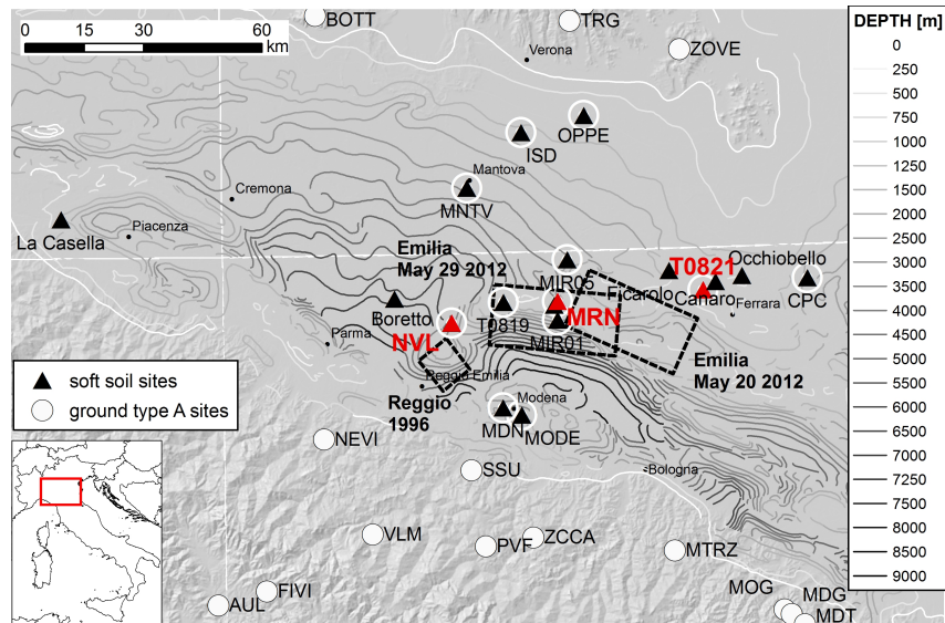
Figure 1. DEM of Po Plain area with sites of interest, showing also depth contours of the base of Pliocene (from Bigi et al., 1992). Rupture area projections of the Reggio 1996 and the two Emilia 2012 mainshocks are also displayed as black rectangles. S
