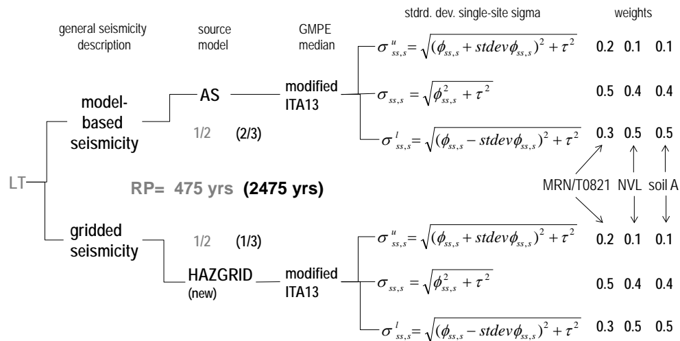
Figure 4 – Logic Tree for SH computations. “Modified ITA13” refers to Equation (1). Weights assigned to sigma level branches are shown on the right. Weights of the source model were changed from 475 to 2475 yrs, because the gridded seismicity model reflects the earthquake catalogue completeness period, not exceeding 500-1000 yrs for the higher magnitudes.
