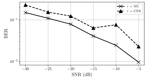
FIGURE 16. SNR versus BER for NN and CNN.
