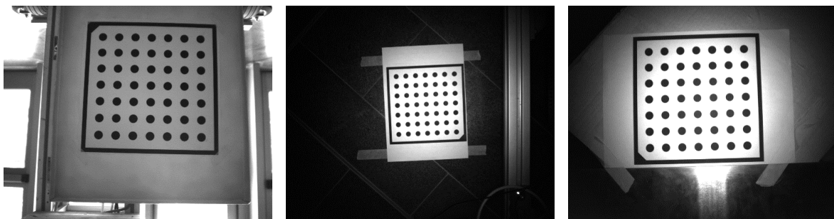
Figure 15. Laviw internal calibration of the on-board cameras
