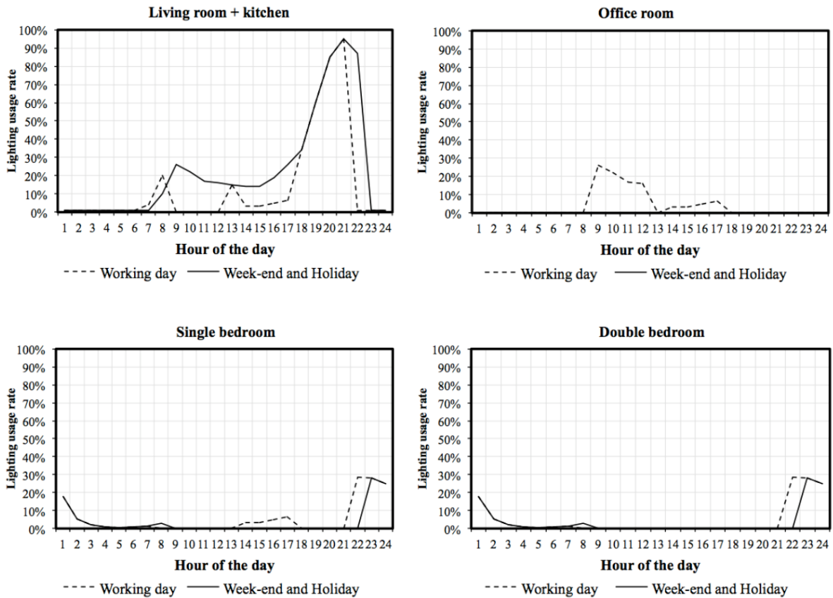
Figure A-2: Daily schedule for lighting.
