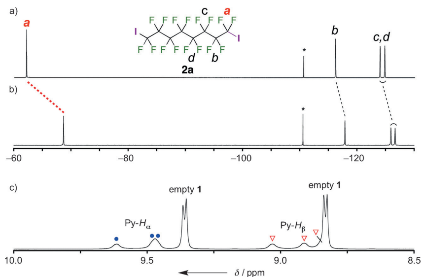
Figure 2. a,b) ^{19}\text{F} NMR spectra (470 MHz, 300 K) of 2a in \text{CDCl}_3 (a) and 1\cdot(2a)_2 in \text{D}_2\text{O} (b; * labels denote signals of the internal standard, 1,3,5-trifluorobenzene, in a capillary tube). c) Expanded ^1\text{H} NMR spectrum (500 MHz, 285 K) of the inclusion complex 1\cdot(2a)_2 in \text{D}_2\text{O} .
