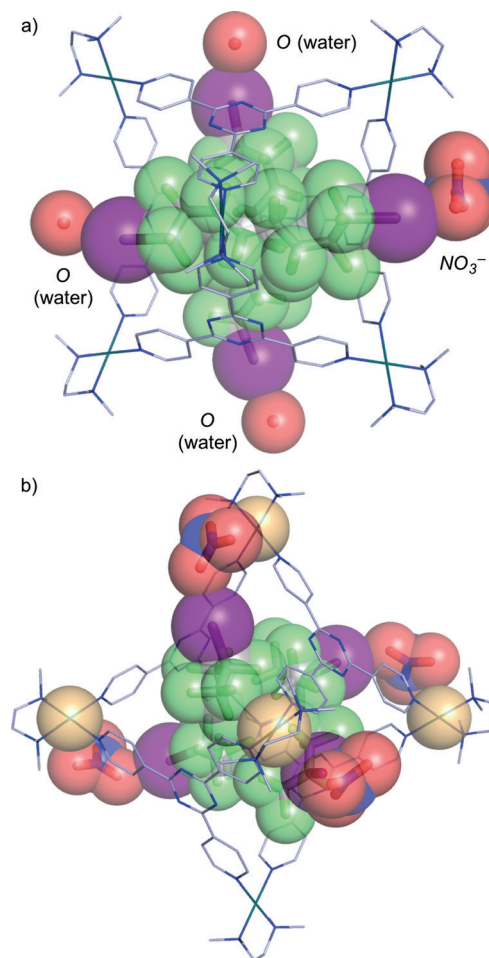
Figure 3. X-ray single-crystal structures of a) 1\cdot(2a)_2 and b) 1\cdot(2e)_4 (C gray, N blue, O red, F green, I purple, Pd brown). H atoms, \text{NO}_3^- anions, and water molecules that are not involved in halogen bonding have been omitted for clarity. Only one of the disordered structures is shown for 1\cdot(2e)_4 .
