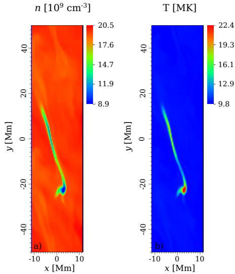
Fig. 5.— Slices of the z = 0 plane for Model M4 with a pressure pulse diameter of 4Mm, at t = 50.3 min: a) number density, n and b) temperature, T . See also the movies attached to the electronic version of the paper.
