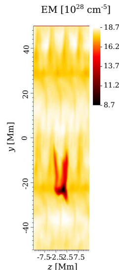
Fig. 8.— Face-on CS view of the EM for model M4 , pulse size of d = 4 Mm, at t = 50.3 min.
