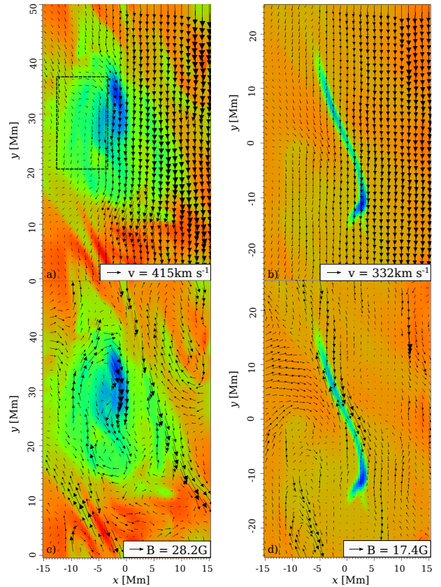
Fig. 6.— Velocity of the z = 0 view for models a) M1 at t = 20 min and b) M4 at t = 49.4 min. Magnetic field of the z = 0 view for models c) M1 at t = 20 min and d) M4 at t = 49.4 min. The arrows inserted represent values at the scale of the vector fields for the magnitude immediately to the lower right corner.
