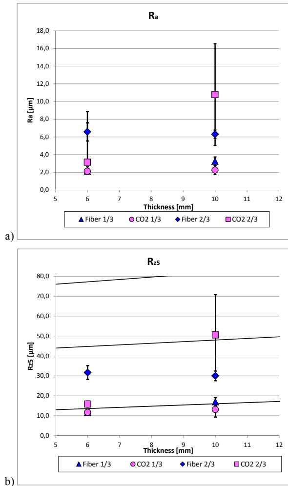
Fig.2. Summary of a) R_a and b) R_{z5} for the analyzed stainless steel samples.
