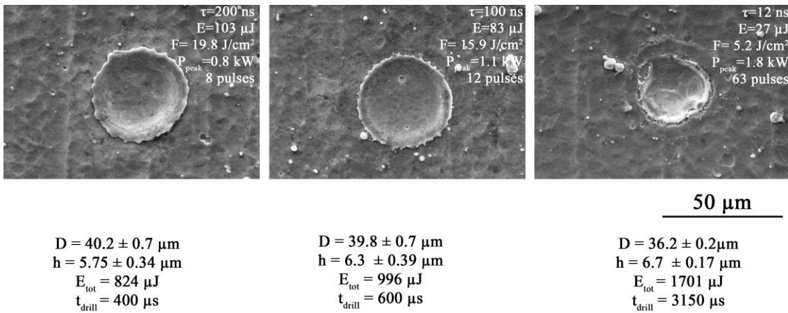
Figure 6. A comparison of holes with similar geometric properties obtained with different pulse durations, energy levels and number of pulses.
