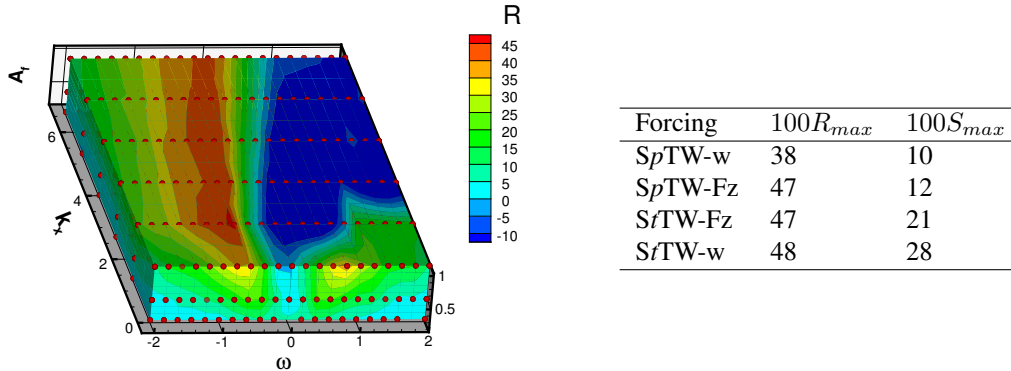
Figure 1. Left: example result, map of R for StTW-Fz with \Delta = 0.03 . Right: maximum drag reduction R_{max} and maximum net energy saving S_{max} for the whole parameter study, relative to each forcing type, ordered for increasing S_{max} . Note that in defining R_{max} points at very high A^+ available in the literature for StTW-w and resulting in slightly larger R (up to relaminarization) have been excluded, as the main focus here is on comparison and the present study does not consider extremely high forcing intensities.
