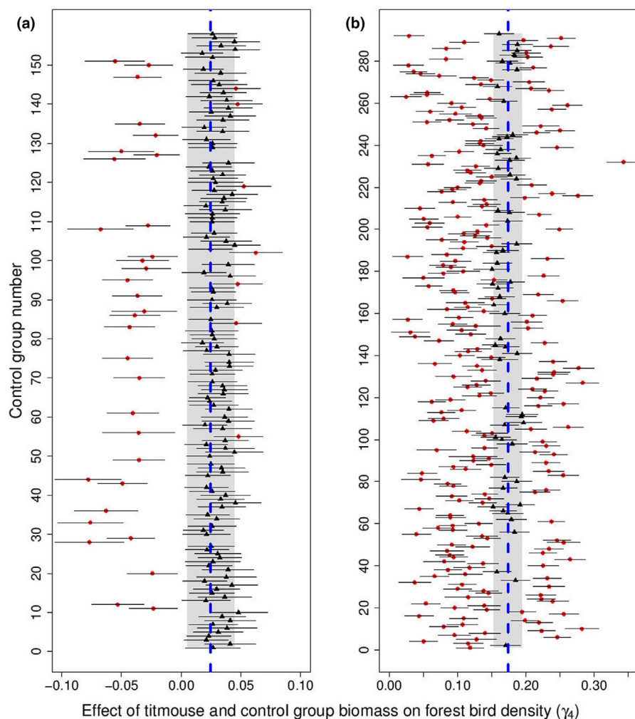
FIGURE 3 VAST estimates from the models that converged and had a significant parameter estimate (a: n = 158 ; b: n = 293 ) for the associations between abundance (given as biomass) of each randomly drawn control group and forest bird density ( \gamma_4 ) with error bars showing the 95% confidence intervals in Finland (a) and in France (b). Red filled circles represent those estimates that were statistically different from the titmouse estimate ( \gamma_1 ; a: n = 39 ; b: n = 235 ) and the black triangles depict those estimates that were not significantly different from the titmouse estimate (a: n = 119 ; b: n = 58 ) at 95% confidence level (see Section 2.4 for details). The estimate for the association between titmouse abundance (given as biomass) and forest bird density is shown with the blue dashed line (a: \gamma_1 = 0.025 ; b: \gamma_1 = 0.174 ), and the gray shaded area shows the 95% confidence intervals for the titmouse estimates
