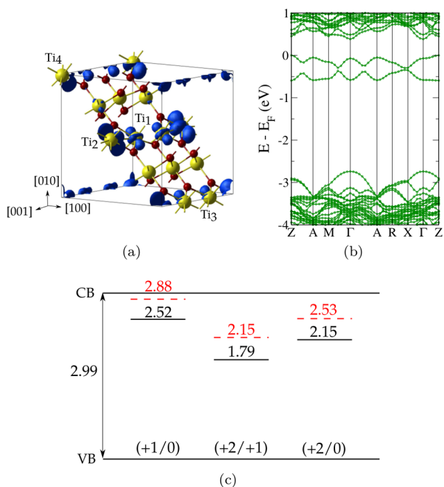
FIG. 1. O vacancy in rutile \text{TiO}_2 . (a) Isosurface plot of the charge density associated with the excess electrons for the neutral vacancy. The yellow (large) and red (small) spheres represent Ti and O atoms, respectively. Only the atomic plane containing the O vacancy is shown. (b) Corresponding electronic band structure (only spin majority is shown) computed at the equilibrium geometry. (c) Optical (solid, black) and thermodynamic (dashed, red) charge-transition levels. Positions (in eV) are given with respect to the top of the valence band (VB).
