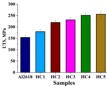
Figure 9: Ultimate tensile strength plot.
