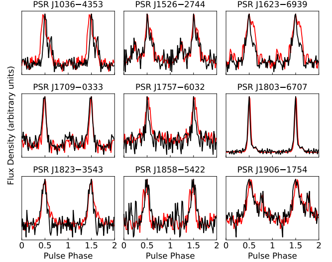
Figure 2. Pulse profiles of the newly-discovered millisecond pulsars. Black and red curves show the profiles from L-band and UHF observations respectively. For clarity, two identical pulses are shown, and pulses have been arbitrarily normalised and phase shifted to peak at phase 0.5.
