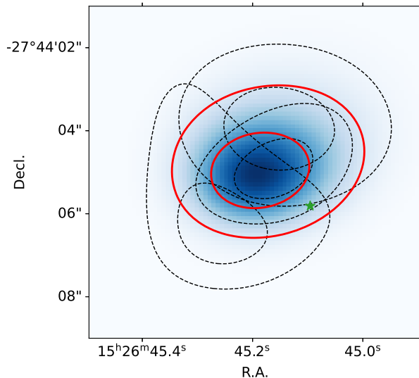
Figure 3. An example of pulsar localisation using SeeKAT, from the three confirmation observations of PSR J1526–2744. The dashed black contours show the localisation probabilities in three separate observations. The colour scale and the solid red contour lines show the joint likelihood (i.e. the product of the likelihoods from all three observations). Contour lines are at approximate 1\sigma and 2\sigma levels. The green star is at the Fermi timing position for this pulsar.
