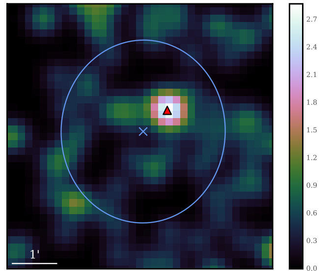
Figure 8. eRASS1 image in the 0.2 – 2.3 keV band, with the 95% positional error ellipse of 4FGL J1803.1–6708 indicated in blue, and the GAIA position overlaid on the eROSITA counterpart of PSR J1803–6707 marked in red. The image has been spatially binned to a pixel size of 10'' and smoothed with a 15'' kernel. The color bar indicates the count rate in units of 10^{-3} \text{ ct s}^{-1} \text{ pix}^{-1} .
