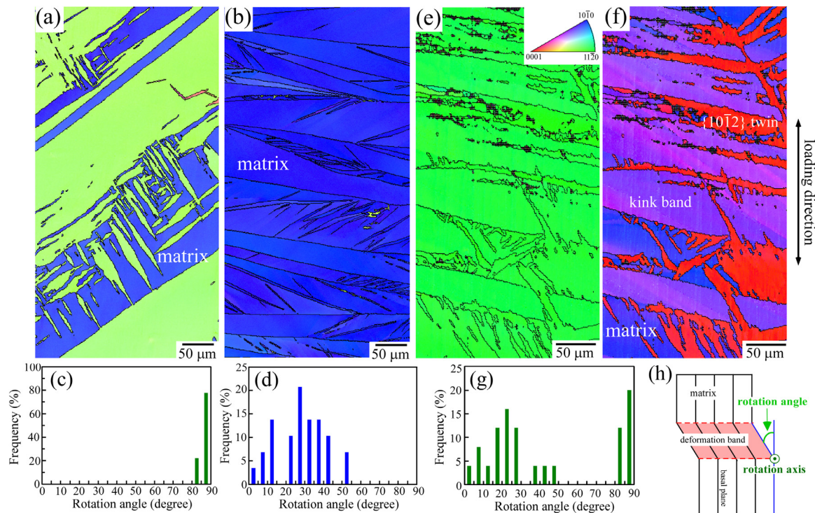
Fig. 5. (a, b) Crystal orientation maps of deformation microstructures of the specimen deformed in the [11\bar{2}0] orientation at RT to ~5% plastic strain and observed on the (1\bar{1}00) side surface. (c, d) Distributions of the crystal rotation angle in the deformation bands with respect to the matrix (undeformed region), measured in the regions around Fig. 5(a) and (b), respectively. (e) Crystal orientation map of the specimen deformed in the [01\bar{1}0] orientation at RT to ~5% plastic strain and observed on the (\bar{2}110) side surface. (f) The same region in Fig. 5(e), but the colors in the map indicate the crystal orientation along the loading axis, in order to distinguish the orientation colors of the deformation twins and deformation kink bands. (g) Distribution of the crystal rotation angle in the region around Fig. 5(e). The colors of the bar graph of Figs. 5(c), (d), and (g) indicate the crystal rotation axis of the measured bands: green: near \langle 2\bar{1}10 \rangle and blue: near \langle 1\bar{1}00 \rangle with a deviation-angle tolerance of 10^\circ . (h) Schematic showing the definitions of the crystal rotation angle and crystal rotation axis in the deformation band.
