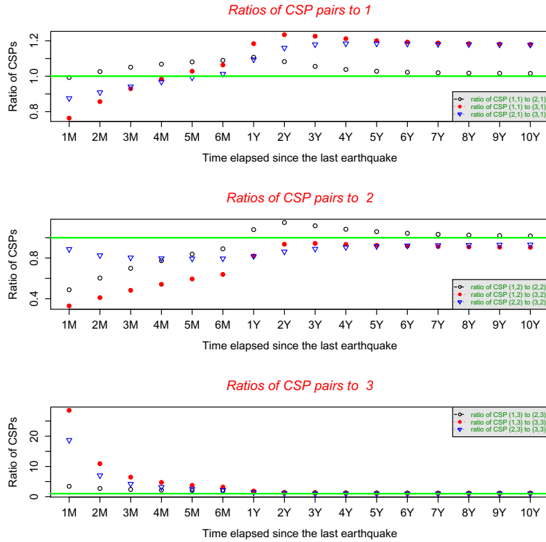
FIG 6. Checking the SPM: posterior means of ratios of CSPs P_{0|\Delta x}^{ij}/P_{0|\Delta x}^{kj} , with time origin at 0, up to 10 years ahead. Transitions are from state 1, 2 and 3 to state 1, 2 or 3. Green horizontal lines at one indicate the theoretical value of the ratios for the SPM. The prior distribution is noninformative.
