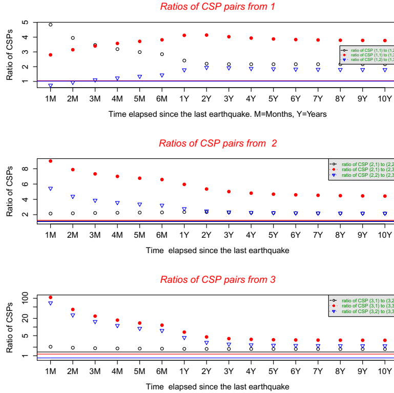
FIG 5. Checking the TPM: posterior means of ratios of CSPs P_{0|\Delta x}^{ij}/P_{0|\Delta x}^{ik} , with time origin at 0, up to 10 years ahead. Transitions are from state 1, 2 and 3 to state 1, 2 or 3. Horizontal lines indicate the theoretical values of the ratios for the TPM. The prior distribution is noninformative.
