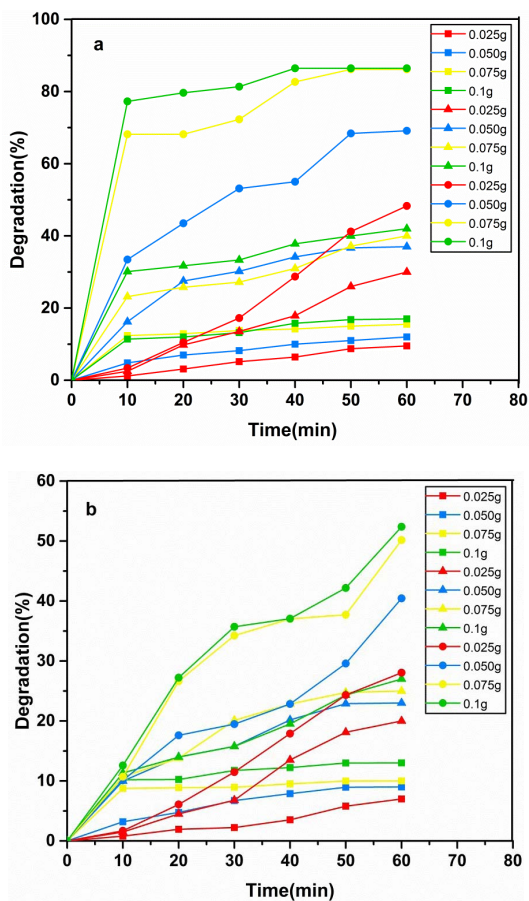
Figure 6. The degradation percentage of Coomassie blue G-250 for various amounts of ■ NiFe 2 O 4 , ▲ ZnO, and • NiFe 2 O 4 /ZnO under (a) UV light and (b) visible light.
