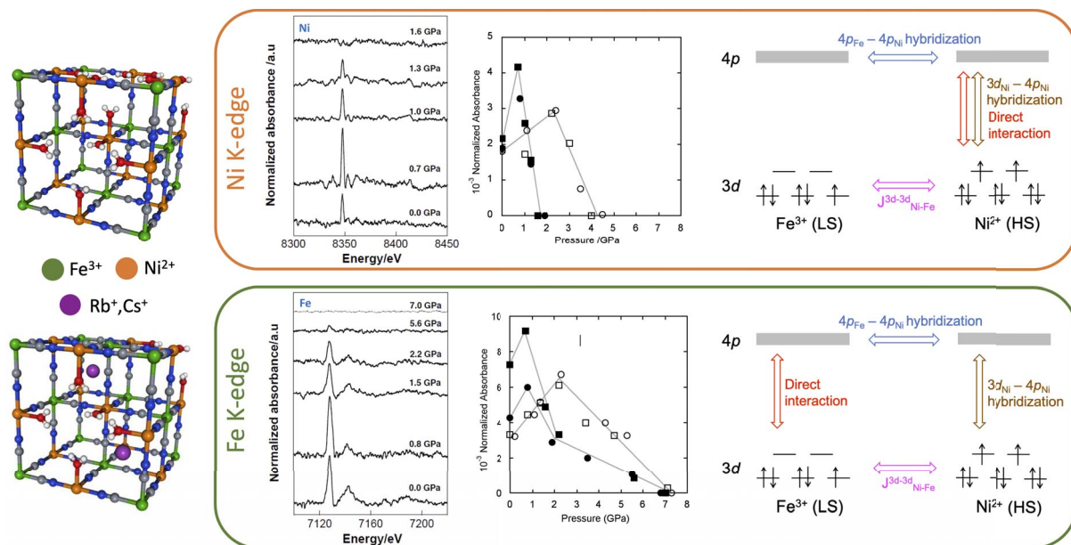
Figure 2. Scheme of the unit cell for the \text{Ni}_4[\text{Fe}(\text{CN})_6]_{2.7} PBA and the \text{Y}_2\text{Ni}_4[\text{Fe}(\text{CN})_6]_{3.3} PBA. Variable pressure XMCD signals of \text{Ni}_4[\text{Fe}(\text{CN})_6]_{2.7} , variation of the XMCD intensity with pressure for the four PBAs ( \text{Ni}_4[\text{Fe}(\text{CN})_6]_{2.7} = black squares, \text{Cs}_1\text{Ni}_4[\text{Fe}(\text{CN})_6]_3 = black circles, \text{Cs}_2\text{Ni}_4[\text{Fe}(\text{CN})_6]_{3.3} = white squares and \text{Rb}_2\text{Ni}_4[\text{Fe}(\text{CN})_6]_{3.3} = white circles) and scheme of the orbitals and interactions contributing to the signal at the Ni K-edge (upper panel) and at the Fe K-edge (lower panel). Adapted from Ref. [78].
