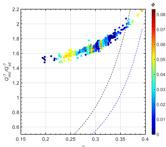
Figure 14. Cross-plot of monopole to dipole attenuation versus Poisson's ratio ( \nu ), color-coded by water content ( \Phi = porosity * water saturation). The blue and black dashed curves were produced from (7) and (8), respectively.
