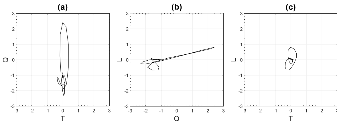
Figure 7. Particle motion of waveforms extracted around the time indicated by the dashed curves in Figure 5. The waveforms are aligned in the direction of L, Q, and T, the components of a ray-based coordinate system which are aligned with P, SV, and SH phase motions. The waveforms are recorded at a depth of 2305 m and an offset of 972 m.
