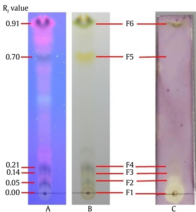
Figure 1. Chromatographic TLC plate of methanolic extract of P. foetida leaves using mobile phase from the mixture of ethyl acetate and n -hexane (7:3 v/v) visualized under (A) UV 366 nm, (B) visible light, and (C) after stained with DPPH reagent in visible light
