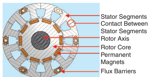
FIGURE 2 – The geometry of the proposed PM design with flux barriers.
