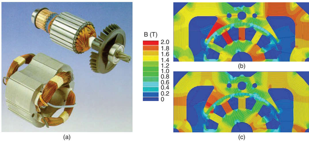
FIGURE 10 – (a) A typical layout of a UM. (b) and (c) FEM analysis of the magnetic core: (b) a standard symmetrical core and (c) the lamination geometry with an asymmetrical yoke and pole shoe widths to reduce local saturation.
