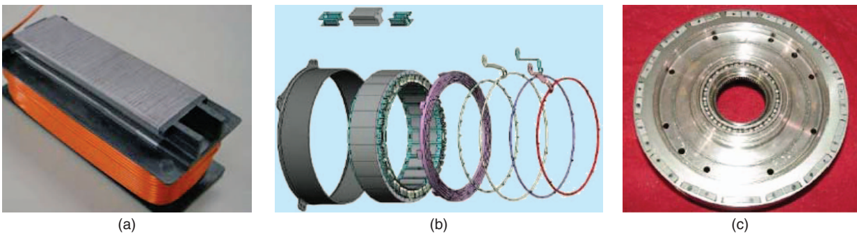
FIGURE 4 – (a) The one-tooth assembly of Chevy Volt's Motor A. (b) Chevy Volt's Motor A assembly diagram. (c) Chevy Volt's Motor A rotor with the end ring removed to show the magnet arrangement [1].
