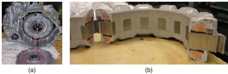
FIGURE 3 – (a) The Prius 2010 FSCW PM generator. (b) A cutout of the Prius 2010 FSCW PM generator stator winding [1].
