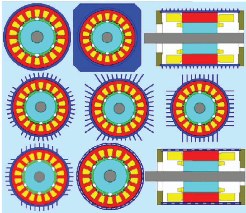
FIGURE 6 – The housing configurations for BPM cooling systems.
