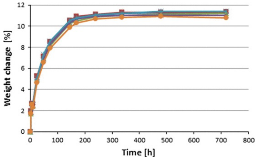
Fig. 9 Water absorption tests.
