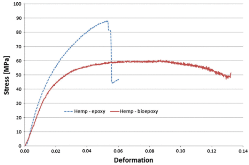
Fig. 10 Resin influence on the toughness of the composite in the bending test.
