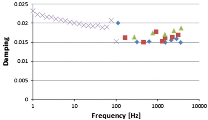
Fig. 11 Damping ratios at all the frequencies tested.
