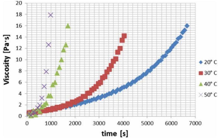
Fig. 7 Curing curves at different temperatures.
