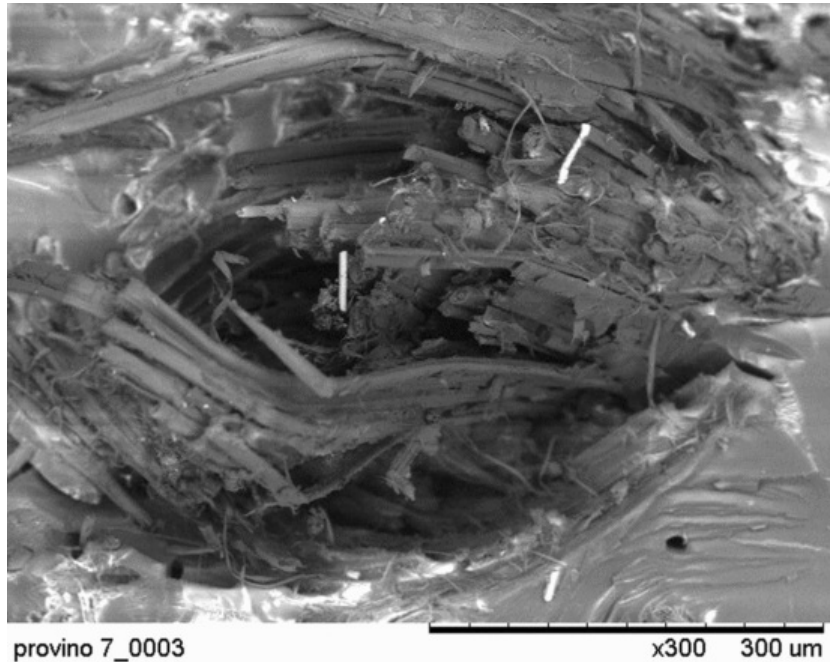
Fig. 12 Fracture surface of a tensile tested laminate.
