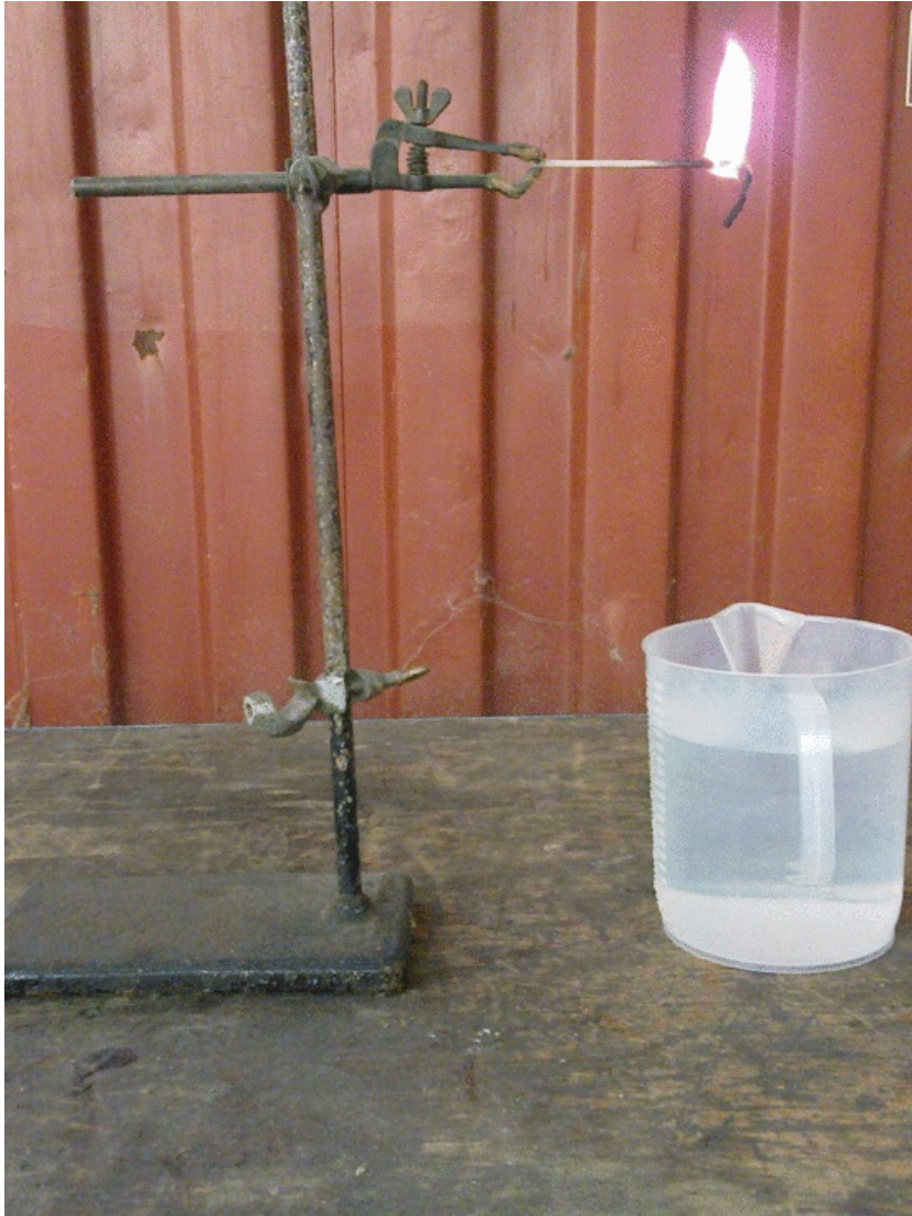
Fig. 6 Flammability test: horizontal set up.
