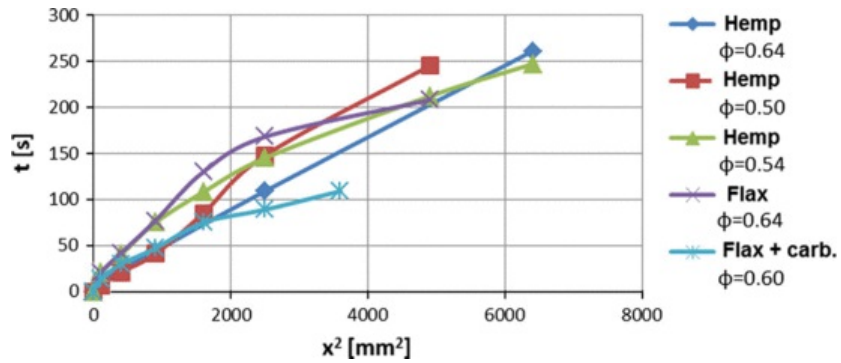
Fig. 8 Comparison of the permeability of the different materials tested.
