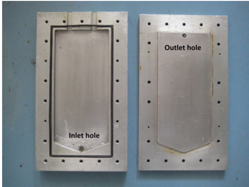
Fig. 3 Composite laminates production mold.
