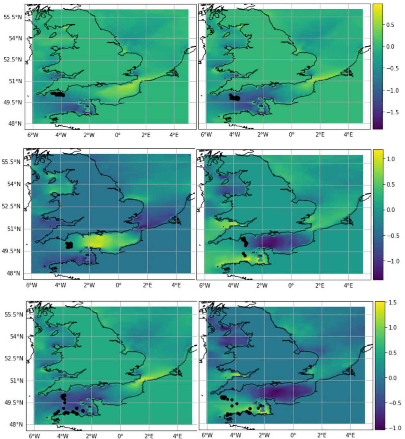
Figure 7. Position of particles backwards in time. Dates move back in time from left to right and top to bottom. Particles were released within a radius of 50 km ( 50^{\circ} 28' 29.1'' \text{N} , -4^{\circ} 22' 7.2'' \text{W} ). The colour bar represents the surface current ( u ) on the last day of the simulation. Simulations are run with Ocean Parcels.
