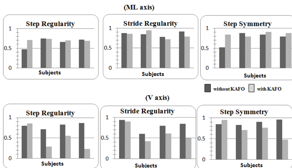
Figure 5. Comparison of step/stride regularity and symmetry evaluated both for the ML and V acceleration sensing axes. Values were normalized and expressed as non-dimensional indexes ranging from 0 to 1. Light grey and dark grey were used to discriminate between the trials carried out with and without the orthosis, respectively.
