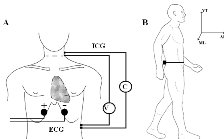
Figure 2. Experimental set-up. (A) Electrode positioning: C is the current injecting electrodes and V the voltage measuring electrodes for the impedance cardiograph while the ECG bipolar derivation is fixed under the sternum; (B) The wearable unit and the acceleration sensing axes (ML: medium-lateral, AP: antero-posterior, V: vertical).
