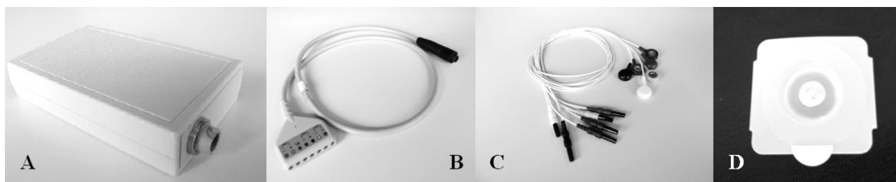
Figure 1. Wearable components of the ECG/ICG/acceleration cardiographic system. (A) Data-logger (117 × 70 × 23 mm); (B) Holter main cable. (C,D) Cable set and Cleartrace ™ adhesive electrodes (ConMed Corporation, Utica, NY, USA).
