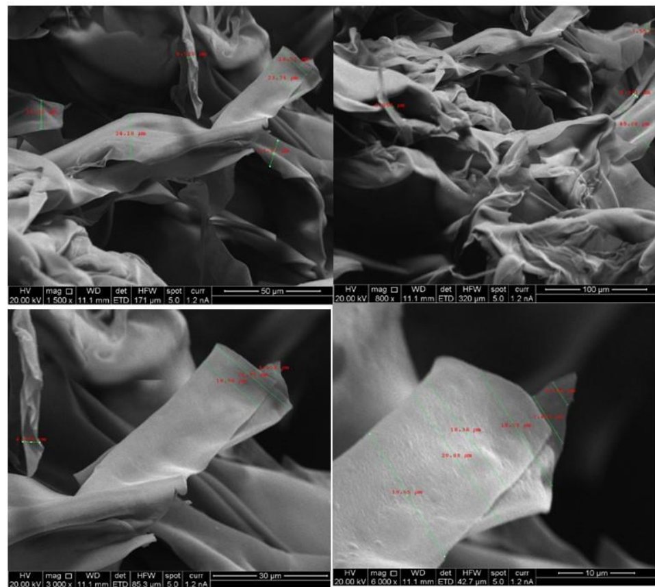
Figure 2. SEM micrograph of chitosan micro-ribbons.
