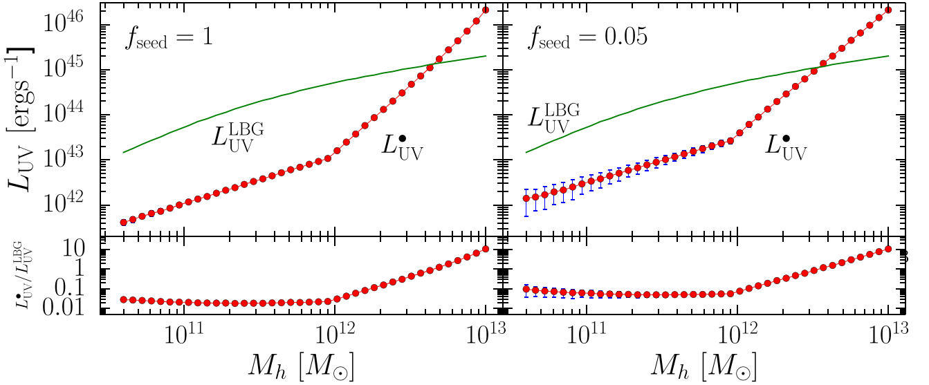
Figure 3. Left: LBG (green line) and BH (red points) UV luminosity versus halo mass for S1. The bottom panel shows the luminosity ratio L_{UV}^{\bullet}/L_{UV}^{\text{LBG}} between the two components across the halo mass range. Variance of individual points is evaluated from \approx 100 merger tree realizations performed per halo mass bin. Right: Same for S2 ( f_{\text{seed}} = 0.05 ).
