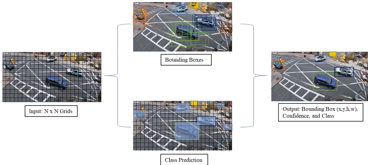
Figure 4 YOLO Algorithm process flow chart
