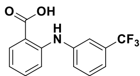
Flufenamic acid
