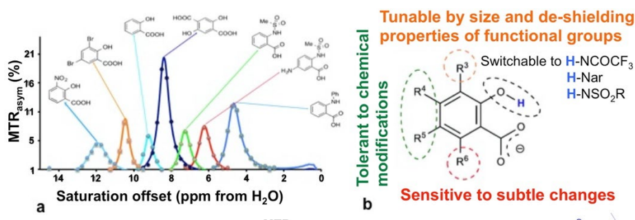
Figure 9. Select salicylate and anthranillate CEST agents. A) 7 of these agents with labile protons resonating between 5 – 12 ppm from water; b) general scaffold for these agents, with MRI properties tolerant to conjugation at R4, R5; Reprinted from Ref 151
