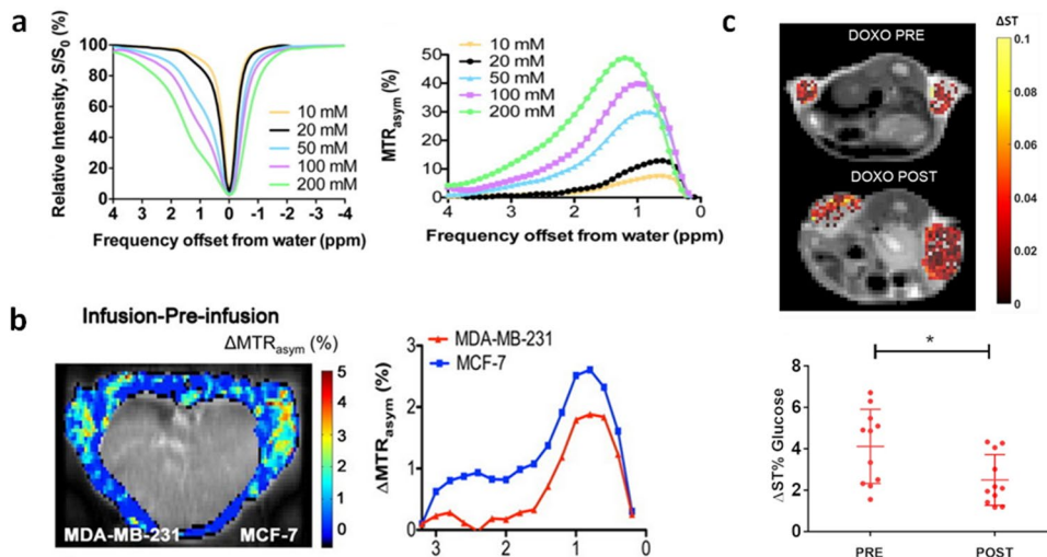
Figure 1. a) Z-spectra (left) and MTR asy (right) as a function of concentration at pH 7.3 for B 1 =1.6 μT. b) Left: GlucoCEST difference map: ΔMTR asy = MTR asy (Infusion)–MTR asy (Pre-infusion). The intensity of the internal body was thresholded out because it contains moving areas (lungs and heart) that have large magnetic susceptibility differences with surrounding tissues, which complicates difference imaging. Tright: the ΔMTR asy profiles of MDA-MB-231 and MCF-7. [Reprinted from 23074027] c) Top: representative glucoCEST ΔST% maps of 4T1 tumor-bearing mice, before and after treatment. Data are reported as the difference (ΔST%) between the ST effect before and after the intravenous glucose injection. Parametric maps are superimposed to T 2w anatomical images and glucoCEST contrast is shown only in the tumor region. Bottom: graph showing individual GlucoCEST contrast (and mean ± SD) obtained injecting glucose at 3 g/kg dose via intravenous bolus (n = 6 mice). Data are reported as the variation (ΔST%) between the ST effect post-injection minus the ST effect pre-injection. Paired t-test *p = 0.0216. [Reprinted from 11 ]
