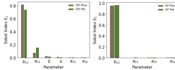
Figure 6. Bar plots of the first-order Sobol index S_1 , for iron concentration in CSF (left) and ISF (right), showing the higher contribution of b_{13} .
