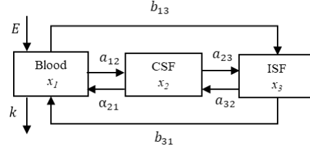
Figure 1. Schematic representation of the barriers forming blood-brain interface, considering blood, CSF and ISF as the three compartments in which the iron concentrations x_1, x_2, x_3 are modulated by the constant E and the parameters listed below.
