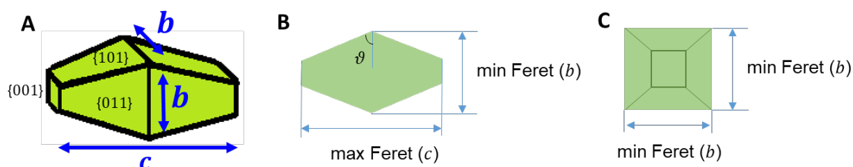
Figure 2. Not-to-scale 3D sketch of a \text{TiO}_2 bipyramid (A), side and top views (B), and front-view (C).
