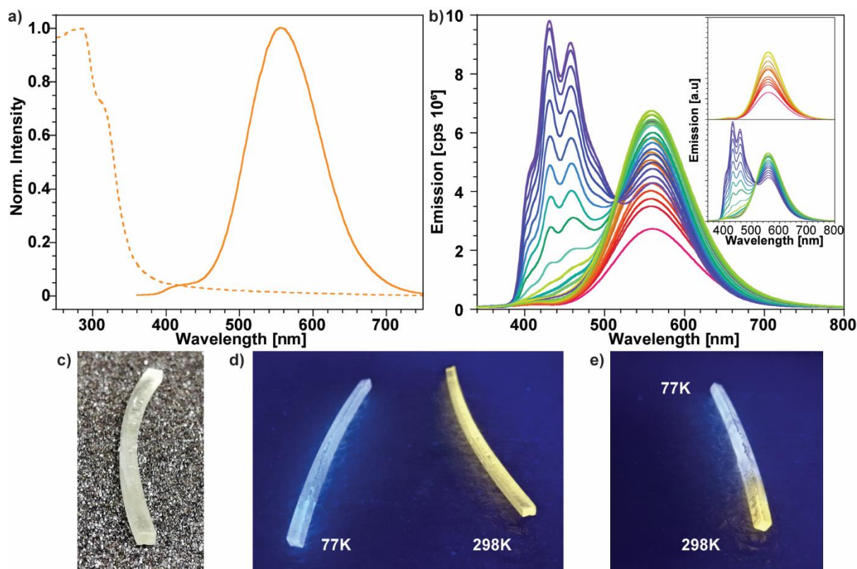
Figure 4. a) Absorption (dashed) and emission (solid) spectra of 3DP film containing 1.0 % of 2. b) Temperature-dependent luminescence spectra of 2 ( \lambda_{\text{ex}} = 330 \text{ nm} , temperature from room temperature to 77 K). The two insets reported the separated first (top) and second (bottom) emission wavelengths. 3DP polymeric waveguide under ambient light (c), under UV (365 nm) light at different temperatures (77 K and 298K) and partially immersed in liquid nitrogen (e).
