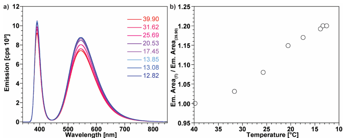
Figure 7. a) Emission spectra at different temperatures for 2 cm length PWG. b) The normalized emission areas at each temperature over the 39.90°C area to demonstrate a reduction in the emitting properties of the PWGs under increasing of temperature.
