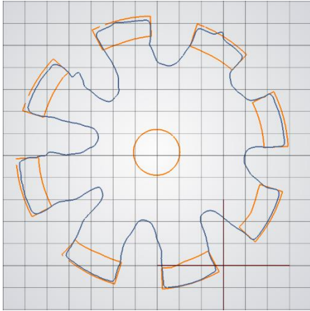
Figure S11. Comparison between a 2D slice of the CAD project (orange) and the 3DP device (blue).
