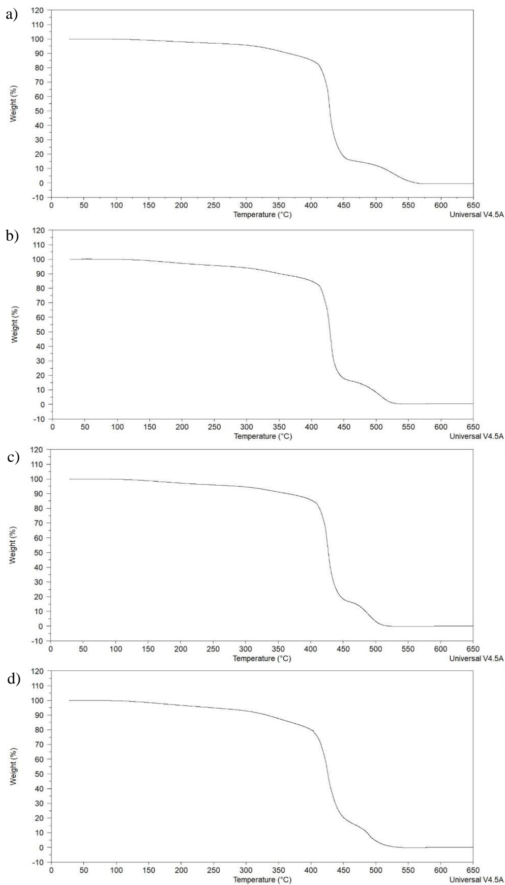
Figure S9. TGA thermograms of 3DP polymeric waveguides with an increasing concentration of 2. a) Blank, b) 0.1 %, c) 1.0 % and d) 5.0 % w -1 .
