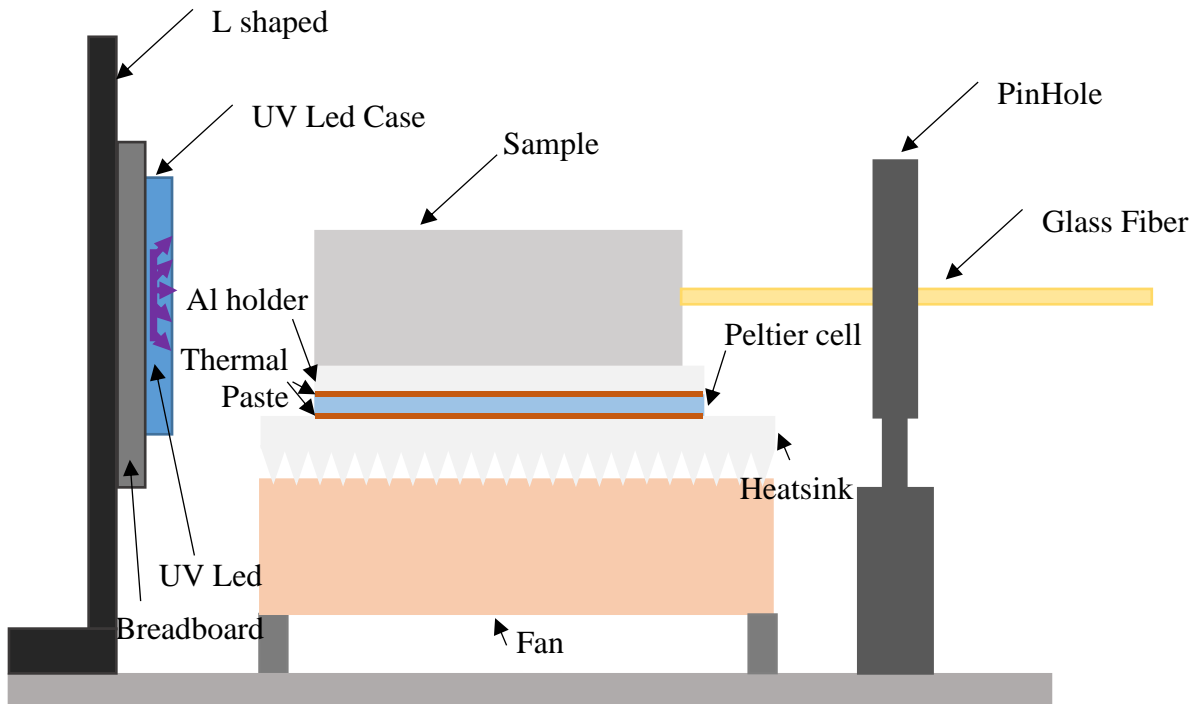
Figure S15. Experimental setup to evaluate the effect of temperature on the emitting properties of PWGs at different lengths.
