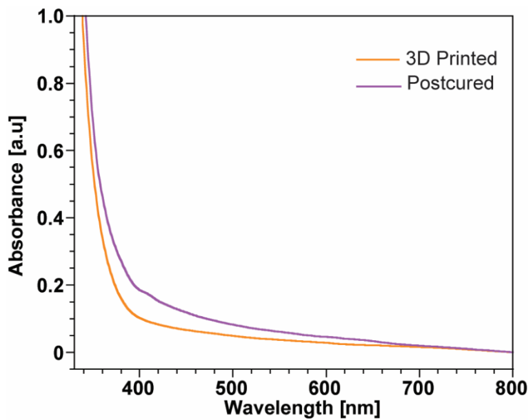
Figure S4. UV-Visible absorption spectra of 3DP polymeric films before and after the post-curing process.
