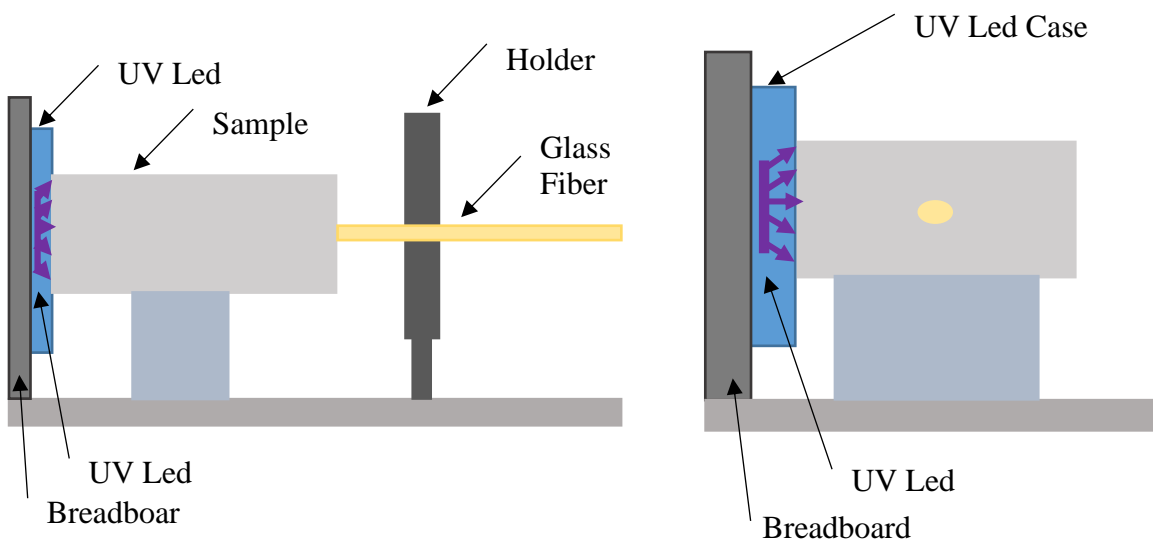
Figure S12. Direct (left) and side (right) pumping experimental configurations to evaluate the emitting properties of the final PWGs.
