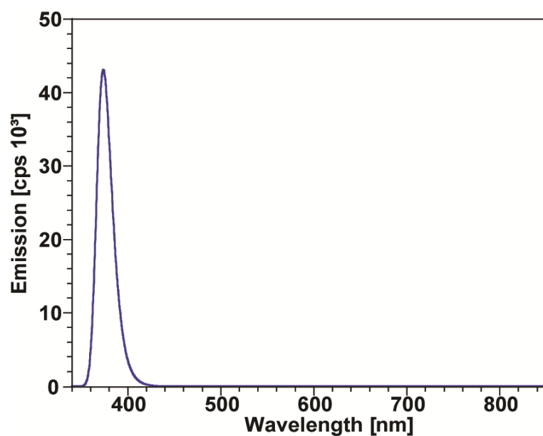
Figure S13. Emission spectrum of UV LED centered at 385 nm.
