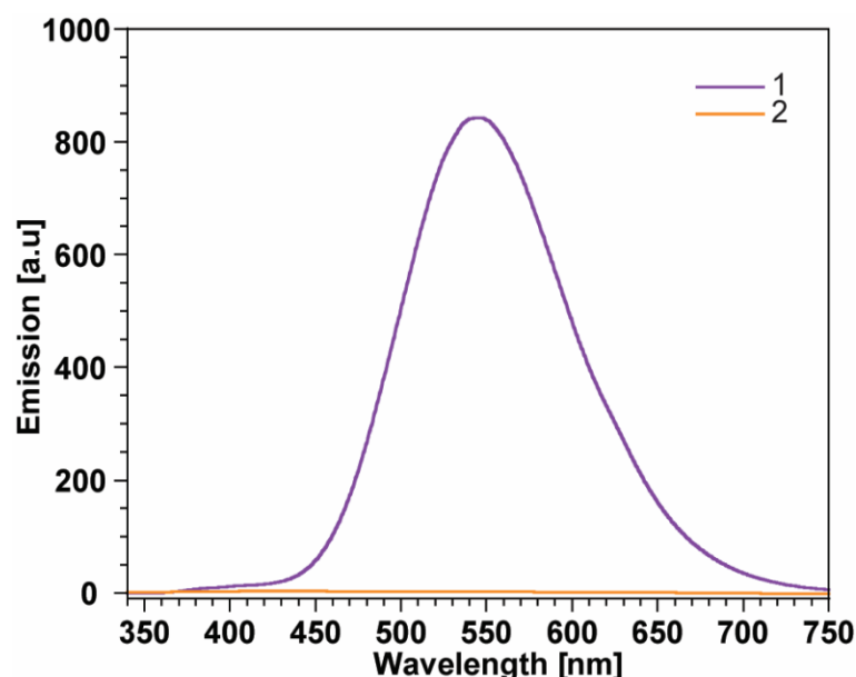
Figure S1. Emission spectra of liquid formulations containing 1.0 % w w-1 of 1 (purple) and 2 (orange). The insolubility of 1 is visible by the emission spectrum, while the totally soluble 2 doesn't emit light (excitation wavelength 330 nm).
