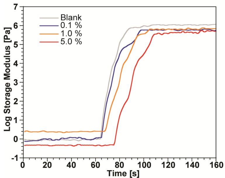
Figure S5. Photorheology tests at 2 % of UV power ( 0.5 \text{ mW cm}^{-2} ) on resins containing increasing concentrations of 2. Blank is the formulation without any copper clusters. A visible delay in the start of photopolymerization reaction is visible in the formulation containing 5.0 % of 2.
