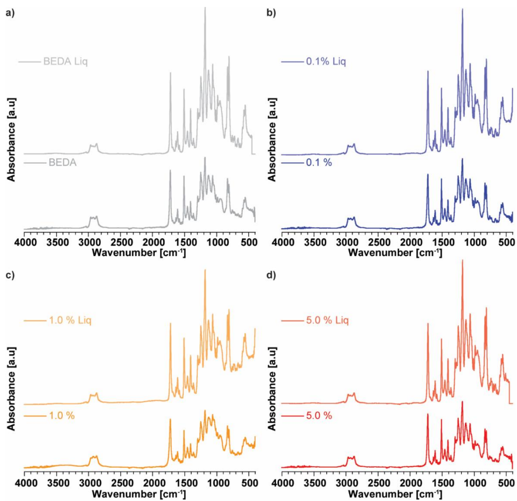
Figure S7. ATR-FTIR spectra of liquid formulation (top) and 3DP post cured films (down) of (a) blank BEDA without copper complex, (b) with 0.1 %, (c) 1.0 % and (d) 5.0 % of 2.
