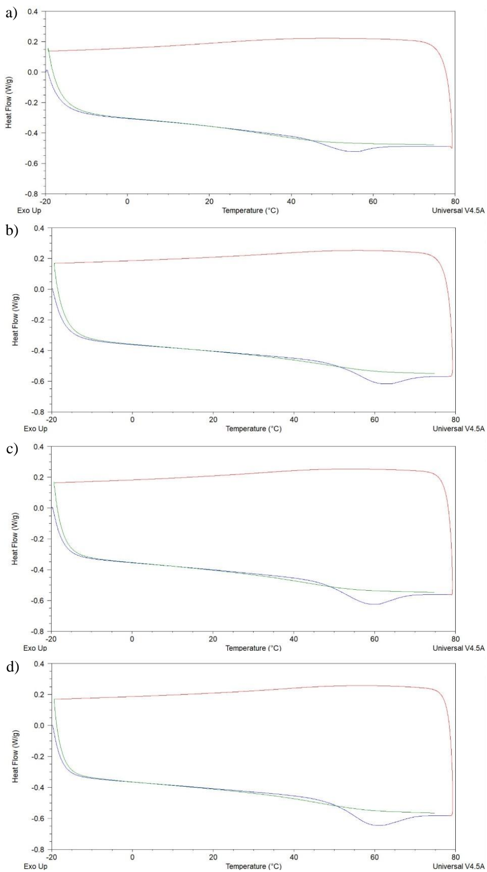
Figure S8. DSC thermograms of 3DP polymeric waveguides with an increasing concentration of 2. a) Blank, b) 0.1 %, c) 1.0 % and d) 5.0 % w w -1 .
