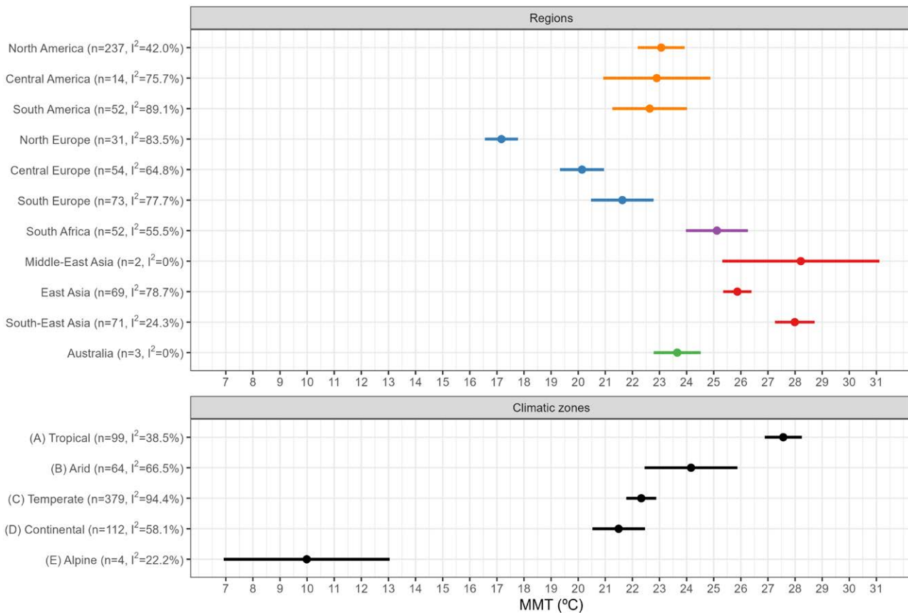
Figure 2. Pooled MMT (°C) by geographical region and Köppen's climatic classification.
