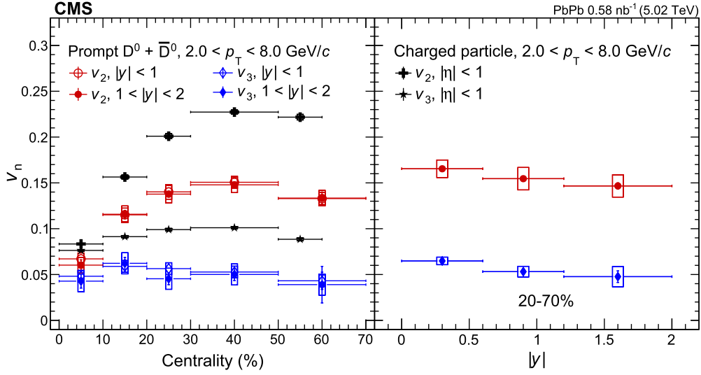
Fig. 4. Prompt D^0 meson v_2 and v_3 as functions of centrality, for 2.0 < p_T < 8.0 GeV/c and for rapidity ranges |y| < 1 and 1 < |y| < 2 . The results are compared with charged particle v_2 and v_3 in the same p_T range and with |\eta| < 1 (left). Prompt D^0 v_2 and v_3 as functions of rapidity, for 2.0 < p_T < 8.0 GeV/c and for centrality 20–70% (right). The vertical bars represent statistical uncertainties and open boxes represent systematic uncertainties. The horizontal bars represent the width of each bin.
