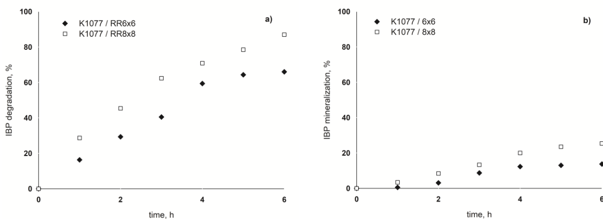
Figure 4: IBP photodegradation (a) and mineralization % (b) over time; comparison between TiO 2 -functionalized 8x8 mm (empty symbols) and 6x6 mm (full symbol) Raschig rings.
