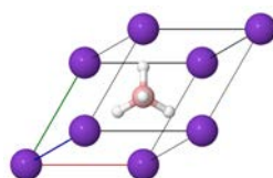
Figure 1: Cell geometry of the face-centered cubic \text{MBH}(\text{D})_4 species ( M=\text{Na},\text{K} )
