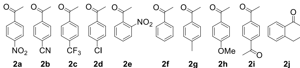
Chart 1: Ketones 2a–j tested in the dehydrative coupling reaction.
