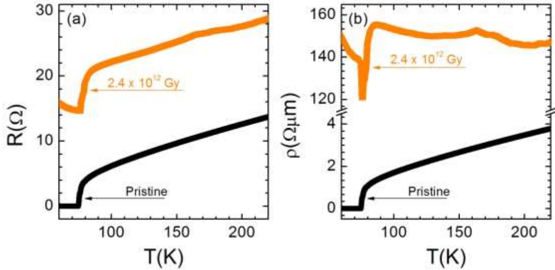
Figure 2. (a) Comparison of the electrical resistance versus temperature behavior, measured for sample A with the four-probe configuration, between the pristine state (black points) and after an X-ray absorbed dose of 2.4 \times 10^{12} Gy (orange points). (b) The electrical resistivity of the irradiated \text{YBa}_2\text{Cu}_3\text{O}_{7-\delta} region (orange points) of sample A is compared to the one of the pristine state (black points). Both behaviors have been calculated from panel (a).
