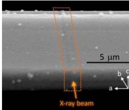
Figure 3. Scanning electron micrograph detail of the \text{YBa}_2\text{Cu}_3\text{O}_{7-\delta} crystal region irradiated with X-rays (sample B). The nanobeam is aligned along the b -axis and scanned in the a - c plane to expose the volume highlighted in orange.
