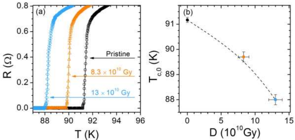
Figure 4. (a) Shift of the resistance transition measured, with a four-probe configuration, in sample B for pristine conditions (black circles) and after the first (orange triangles) and the second (light blue diamond) dose. (b) Critical temperature T_{c,0} vs absorbed dose as determined from panel (a).
