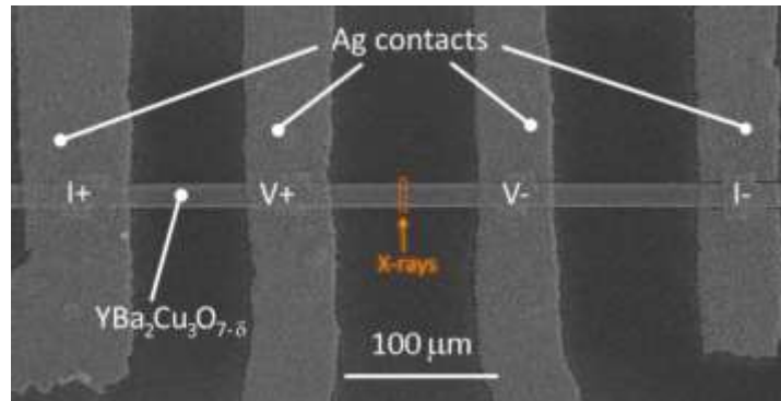
Figure 1 Scanning electron microscope (SEM) image of a typical \text{YBa}_2\text{Cu}_3\text{O}_{7-\delta} electrical device with Ag contacts in four probe configuration. In order to monitor the electrical changes induced by the X-ray irradiation we exposed the region highlighted by the orange rectangle, which is located between the voltage contacts.
