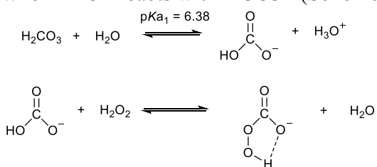
Scheme 2: Mechanism for the formation of peroxy carbonate from carbonate and hydrogen peroxide.
