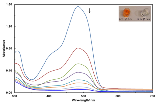
Fig. 10 The change in [O II] from t = 0 to t = 10 min and then at 5 min intervals to 45 min monitored at 484 nm and at 20 \pm 1^\circ\text{C} with [\text{MnCl}_2 \cdot 4\text{H}_2\text{O}] at 5.00 mM. Initial [O II] and [\text{H}_2\text{O}_2] were 0.100 mM and 50.0 mM respectively. The pH was 9.0 \pm 0.1 (50 mM, carbonate buffer). Insert: The colour of O II after attempted oxidative degradation at pH 8.0 (left, no change) and at pH 9.0 (right, completely bleached).
