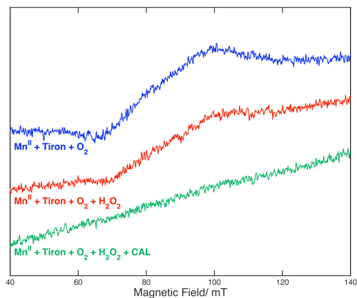
Fig. 4 X-band EPR spectra of MnCl 2 ·4H 2 O (100 mM) and Tiron (~0.30 mM) at pH 8.0 (50 mM, phosphate buffer) followed by the addition of H 2 O 2 (50.0 mM) and then CAL (0.100 mM). EPR conditions: Parallel mode, 9.41 GHz, 10 K, 2 mW microwave power, modulation amplitude 0.5 mT.
