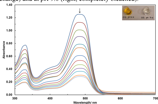
Fig. 11 The change in [O G] from t = 0 to t = 60 min at 5 min intervals to 45 min monitored at 486 nm and at 20 \pm 1^\circ\text{C} with [\text{MnCl}_2 \cdot 4\text{H}_2\text{O}] at 5.00 mM. Initial [O G] and [\text{H}_2\text{O}_2] were 0.100 mM and 50.0 mM respectively. The pH was 9.0 \pm 0.1 (50 mM, carbonate buffer). Insert: The colour of O G after attempted oxidative degradation at pH 8.0 (left, no change) and at pH 9.0 (right, completely bleached).
