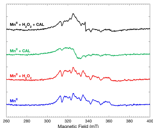
5 Fig. 5 X-band EPR spectra of MnCl 2 ·4H 2 O (100 mM), H 2 O 2 (50.0 mM) and CAL (0.100 mM) at pH 8.0 (50 mM, phosphate buffer) in perpendicular (9.45 GHz) mode. EPR conditions: 10 K, 2 mW microwave power, modulation amplitude 0.7 mT.
