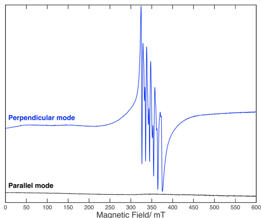
Fig. 3 X-band EPR spectra of MnCl 2 ·4H 2 O (100 mM), H 2 O 2 (50.0 mM) and CAL (0.100 mM) at pH 8.0 (50 mM, phosphate buffer) in both perpendicular (9.65 GHz) and parallel (9.41 GHz) modes. EPR conditions: 10 K, 2 mW microwave power, modulation amplitude 0.5 mT.
