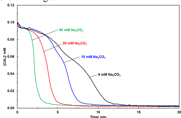
Fig. 9 The change in [CAL] with time monitored at 608 nm and at 20 \pm 1^\circ\text{C} in the presence of Tiron with [Na2CO3] varied from 0 to 50 mM and with [MnCl2·4H2O] at 50.0 mM. Initial [CAL], [H2O2] and [Tiron] were 0.100 mM, 50.0 mM and 1.50 mM respectively. The pH was 9.0 \pm 0.1 (50 mM, N-2-hydroxyethylpiperazine-N'-3-propanesulfonic acid, EPPS, buffer).
