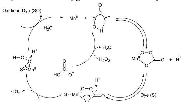
25 Scheme 5 Proposed mechanism for the oxidative degradation of O II and O G via the in situ formation of MnII-O-O-H species.
