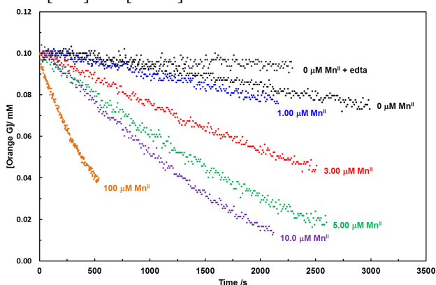
Fig. 13 The change in [O G] with time monitored at 486 nm and at 20 \pm 1^\circ\text{C} with [\text{MnCl}_2 \cdot 4\text{H}_2\text{O}] varied from 0 to 100 \mu\text{M} . Initial [O II] and [\text{H}_2\text{O}_2] were 0.100 mM and 50.0 mM respectively. The pH was 9.0 \pm 0.1 (50 mM, carbonate buffer).
