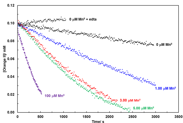
Fig. 12 The change in [O II] with time monitored at 484 nm and at 20 \pm 1^\circ\text{C} with [\text{MnCl}_2 \cdot 4\text{H}_2\text{O}] varied from 0 to 100 \mu\text{M} . Initial [O II] and [\text{H}_2\text{O}_2] were 0.100 mM and 50.0 mM respectively. The pH was 9.0 \pm 0.1 (50 mM, carbonate buffer).
